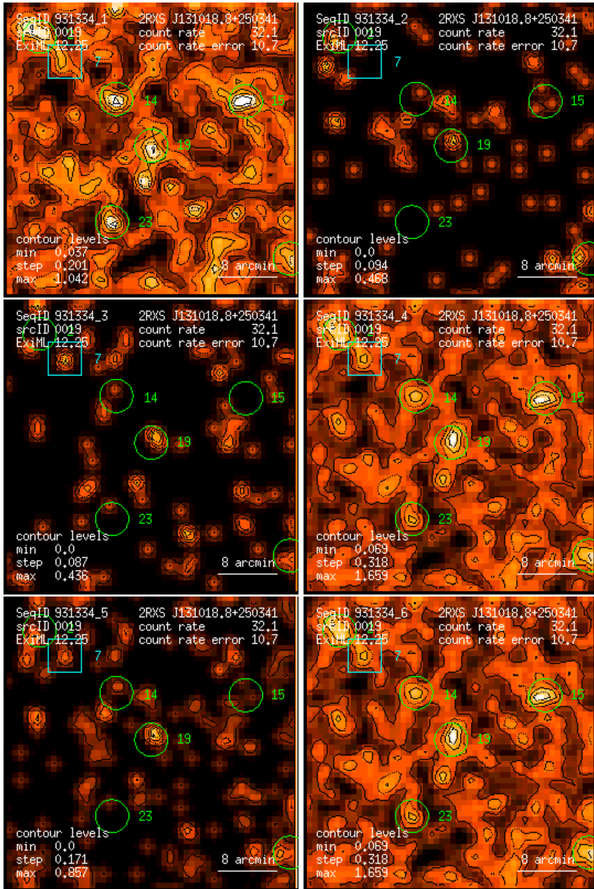
Figure 19: RASS 931334: detection 0019: band rate images, Gaussian filter: (1) PSPC channels 11 – 41, (2) 52 – 90, (3) 91 – 201, (4) 11 – 235, (5) 52 – 201, (6) 11 – 201. Broad band rates in counts/ks. Band rate contour levels in counts/ks/arcmin 2 .
