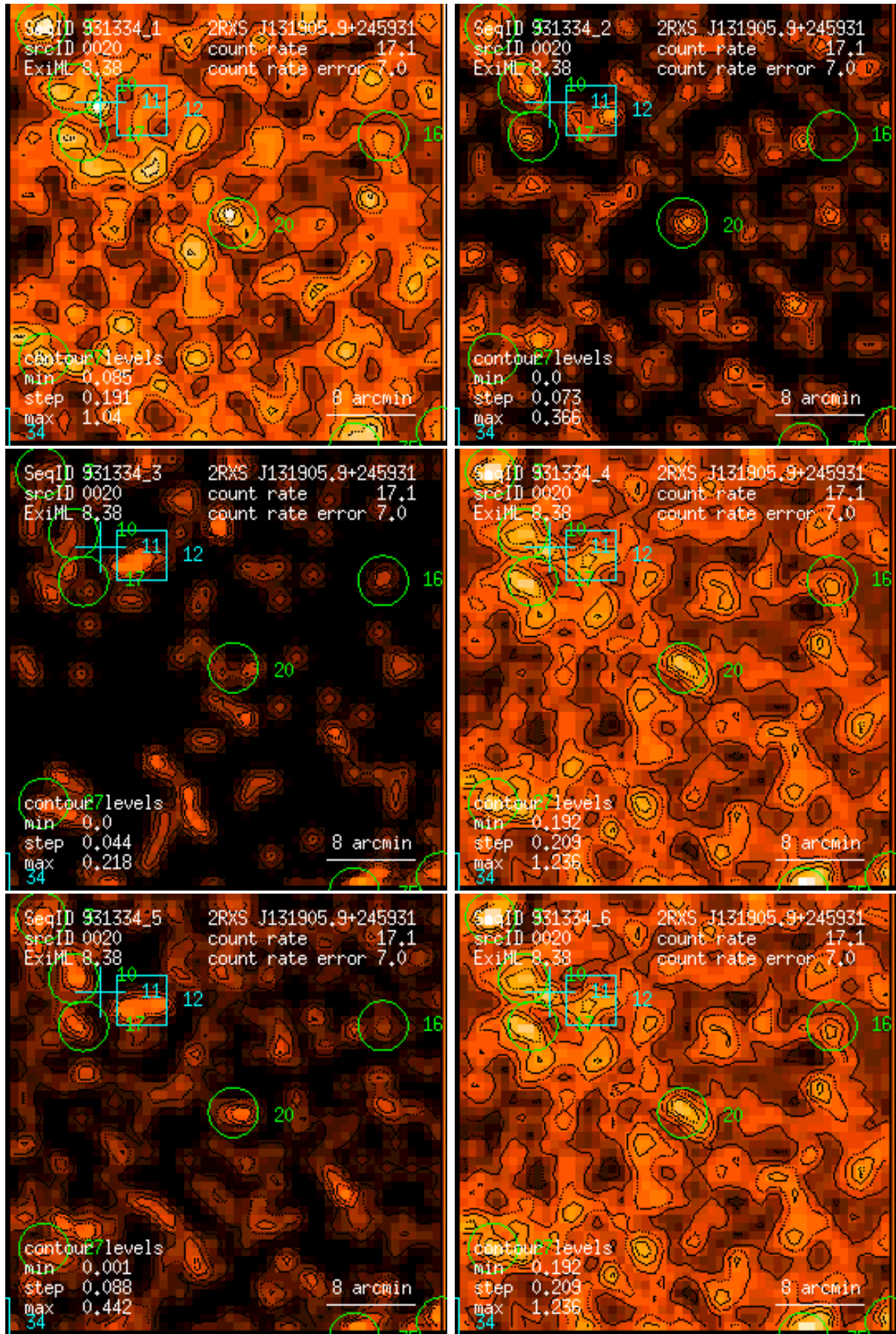
Figure 20: RASS 931334: detection 0020: band rate images, Gaussian filter: (1) PSPC channels 11 – 41, (2) 52 – 90, (3) 91 – 201, (4) 11 – 235, (5) 52 – 201, (6) 11 – 201. Broad band rates in counts/ks. Band rate contour levels in counts/ks/arcmin 2 .
