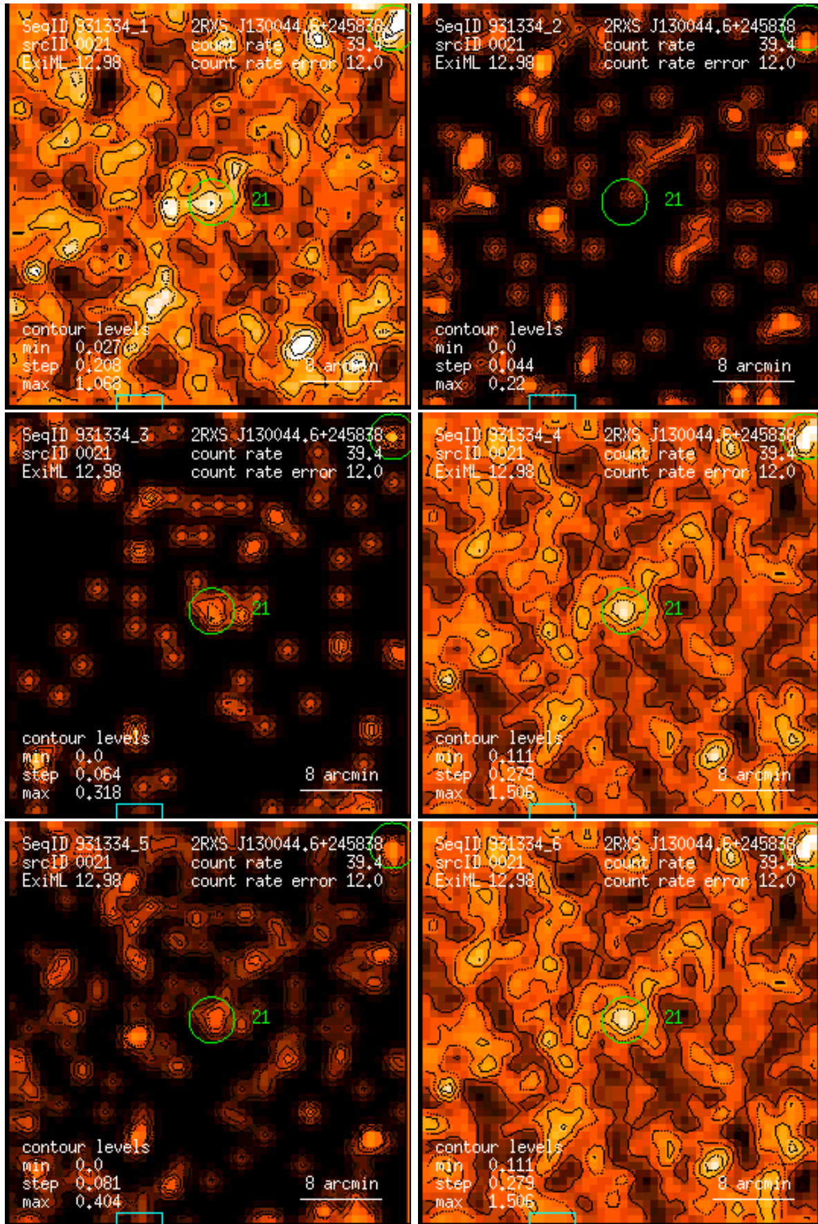
Figure 21: RASS 931334: detection 0021: band rate images, Gaussian filter: (1) PSPC channels 11 – 41, (2) 52 – 90, (3) 91 – 201, (4) 11 – 235, (5) 52 – 201, (6) 11 – 201. Broad band rates in counts/ks. Band rate contour levels in counts/ks/arcmin 2 .
