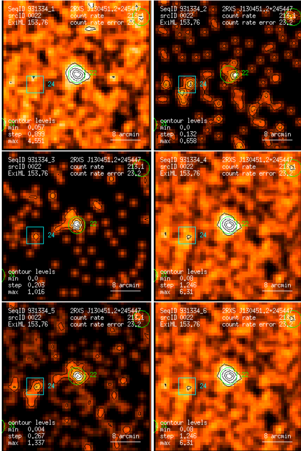
Figure 22: RASS 931334: detection 0022: band rate images, Gaussian filter: (1) PSPC channels 11 – 41, (2) 52 – 90, (3) 91 – 201, (4) 11 – 235, (5) 52 – 201, (6) 11 – 201. Broad band rates in counts/ks. Band rate contour levels in counts/ks/arcmin 2 .
