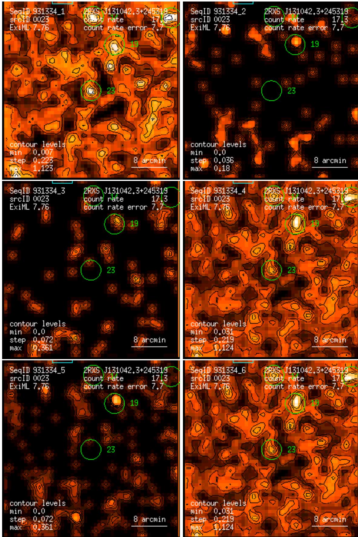
Figure 23: RASS 931334: detection 0023: band rate images, Gaussian filter: (1) PSPC channels 11 – 41, (2) 52 – 90, (3) 91 – 201, (4) 11 – 235, (5) 52 – 201, (6) 11 – 201. Broad band rates in counts/ks. Band rate contour levels in counts/ks/arcmin 2 .
