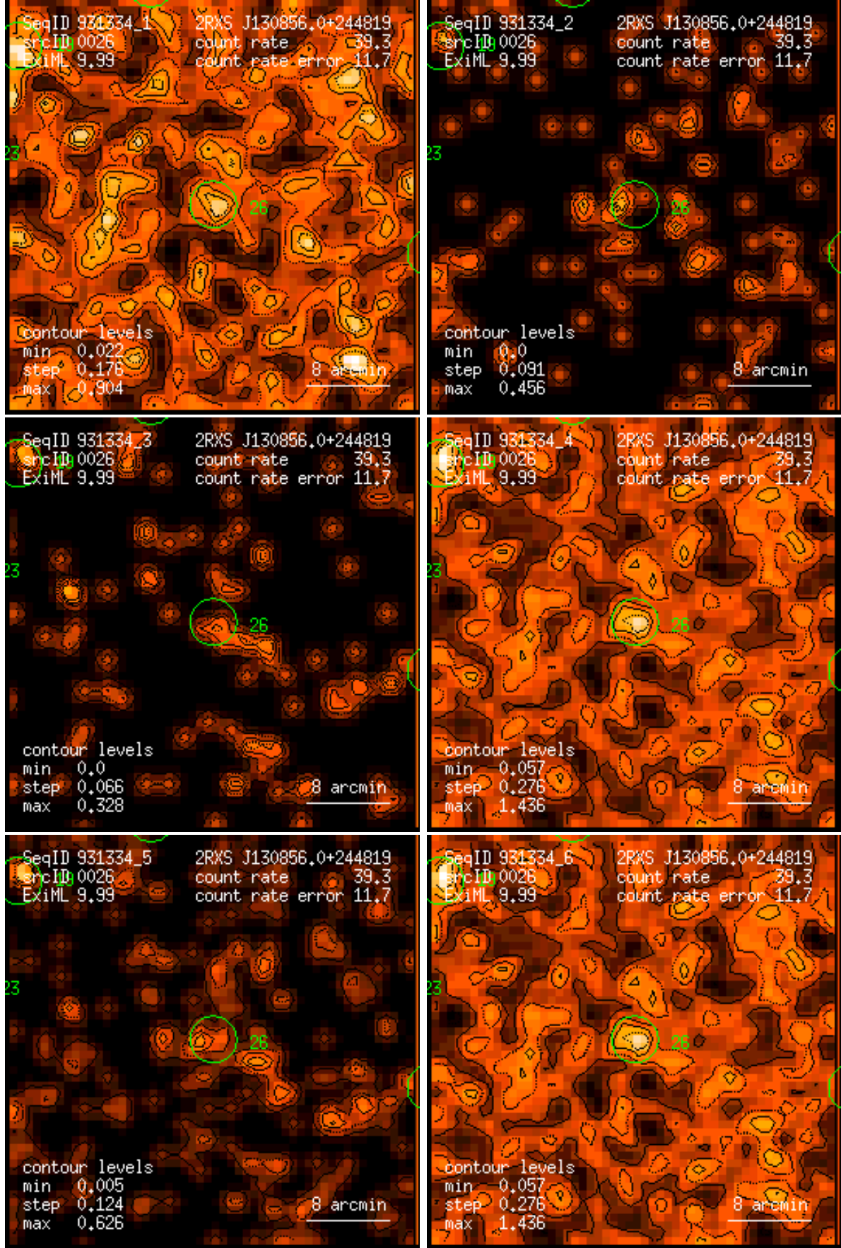
Figure 26: RASS 931334: detection 0026: band rate images, Gaussian filter: (1) PSPC channels 11 – 41, (2) 52 – 90, (3) 91 – 201, (4) 11 – 235, (5) 52 – 201, (6) 11 – 201. Broad band rates in counts/ks. Band rate contour levels in counts/ks/arcmin 2 .
