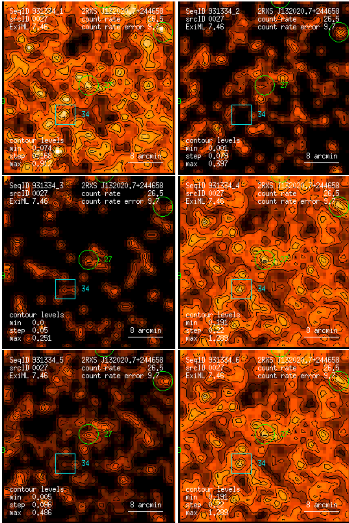
Figure 27: RASS 931334: detection 0027: band rate images, Gaussian filter: (1) PSPC channels 11 – 41, (2) 52 – 90, (3) 91 – 201, (4) 11 – 235, (5) 52 – 201, (6) 11 – 201. Broad band rates in counts/ks. Band rate contour levels in counts/ks/arcmin 2 .
