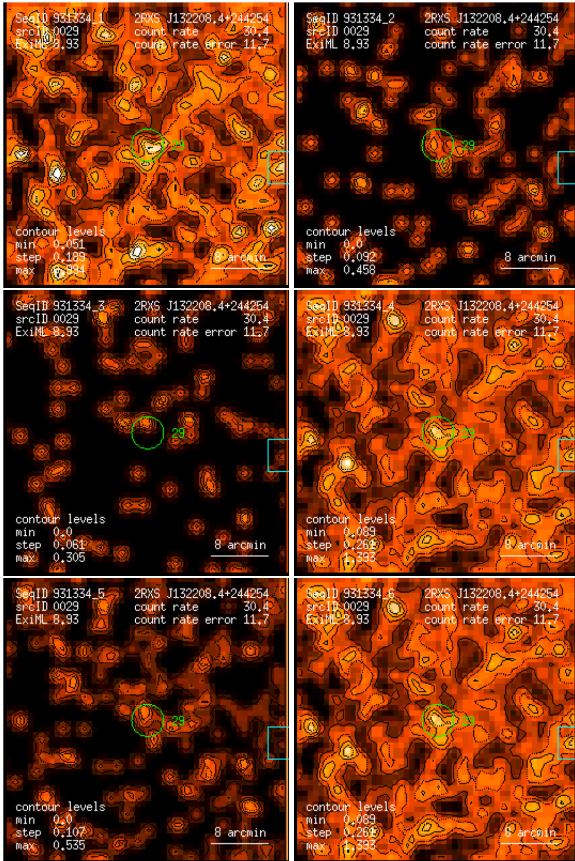
Figure 29: RASS 931334: detection 0029: band rate images, Gaussian filter: (1) PSPC channels 11 – 41, (2) 52 – 90, (3) 91 – 201, (4) 11 – 235, (5) 52 – 201, (6) 11 – 201. Broad band rates in counts/ks. Band rate contour levels in counts/ks/arcmin 2 .
