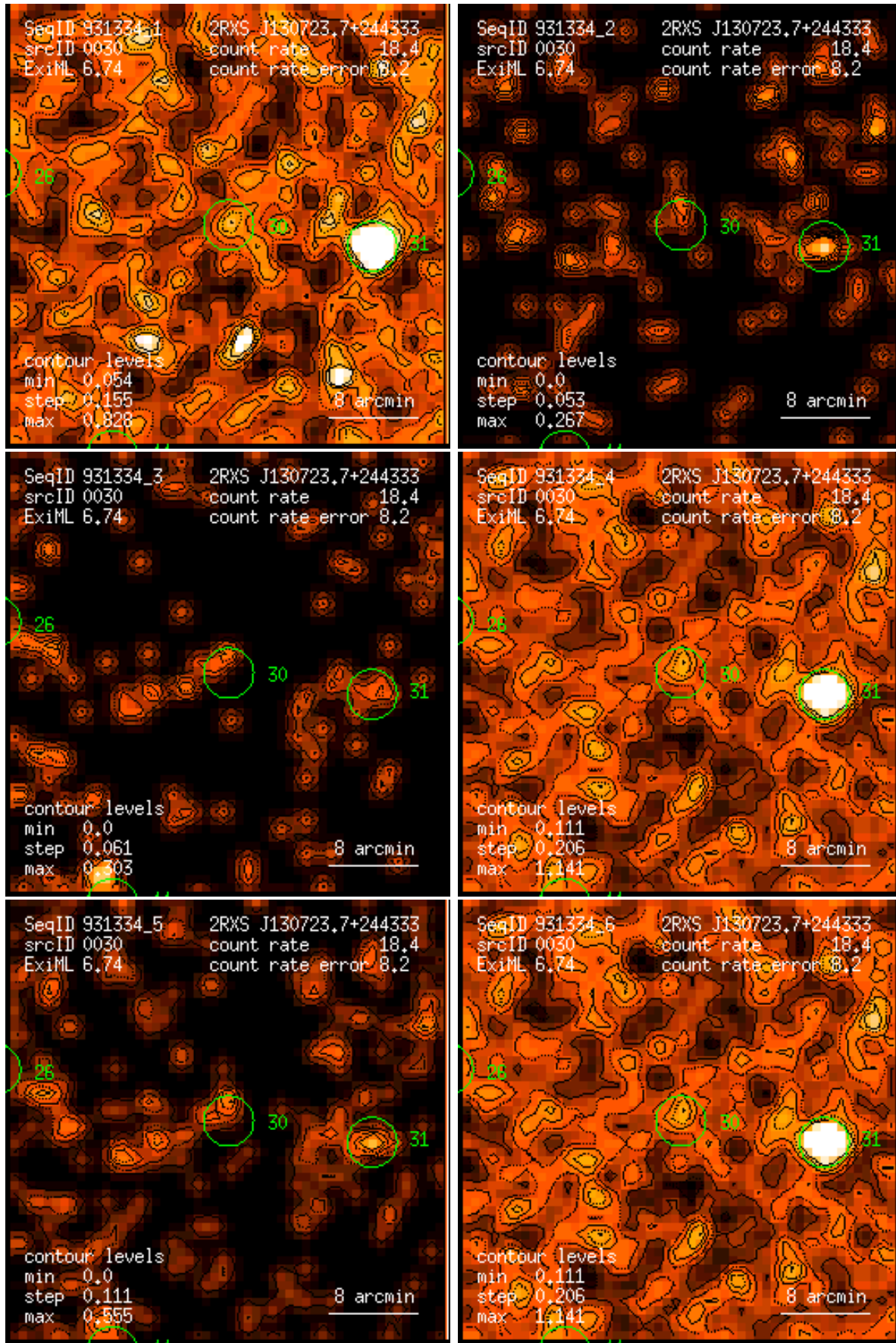
Figure 30: RASS 931334: detection 0030: band rate images, Gaussian filter: (1) PSPC channels 11 – 41, (2) 52 – 90, (3) 91 – 201, (4) 11 – 235, (5) 52 – 201, (6) 11 – 201. Broad band rates in counts/ks. Band rate contour levels in counts/ks/arcmin 2 .
