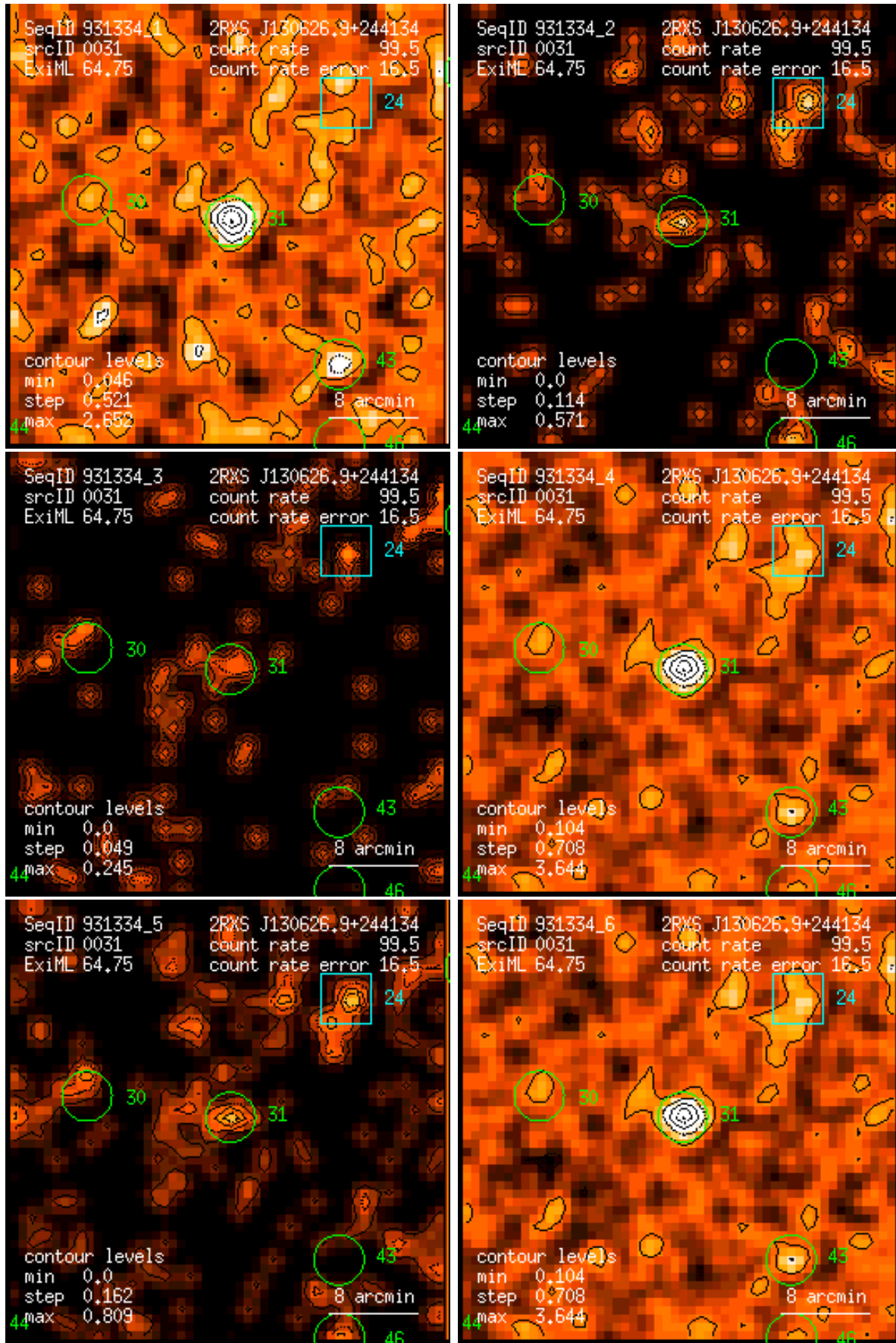
Figure 31: RASS 931334: detection 0031: band rate images, Gaussian filter: (1) PSPC channels 11 – 41, (2) 52 – 90, (3) 91 – 201, (4) 11 – 235, (5) 52 – 201, (6) 11 – 201. Broad band rates in counts/ks. Band rate contour levels in counts/ks/arcmin 2 .
