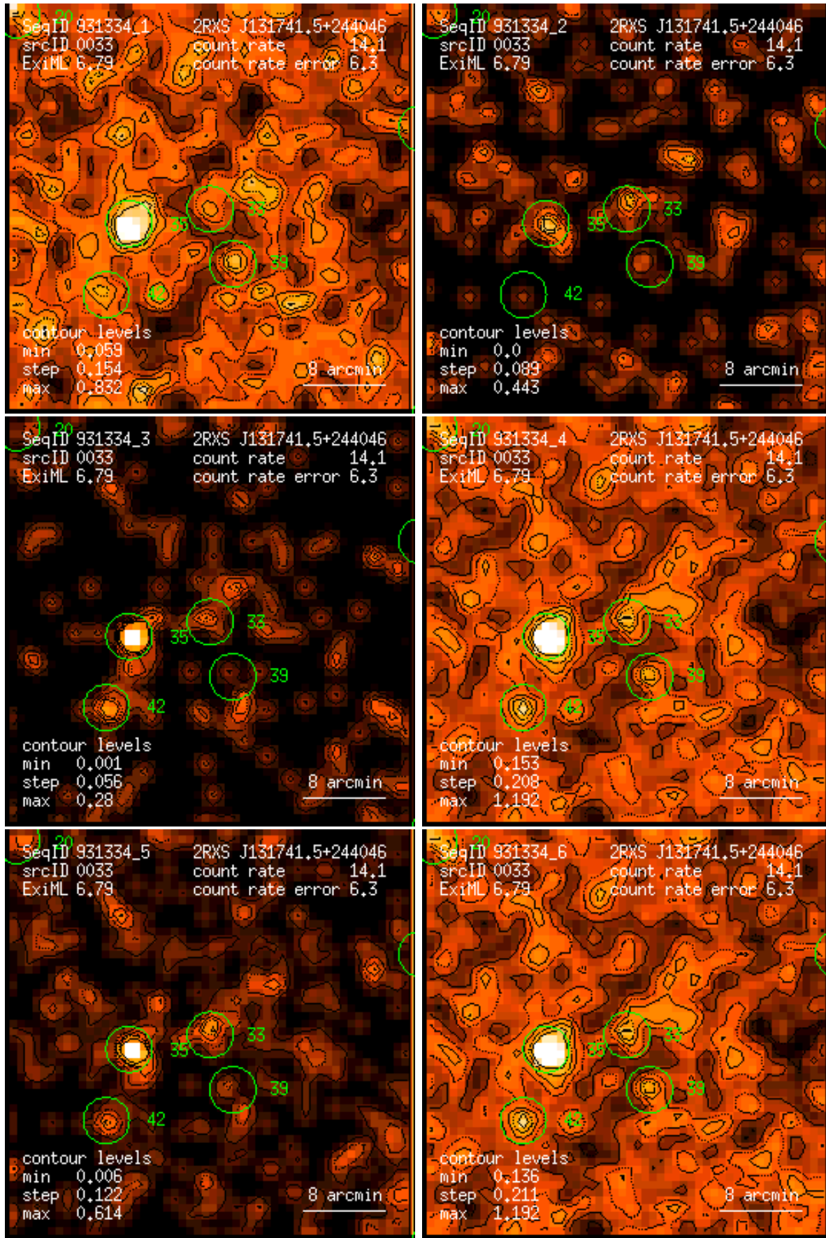
Figure 33: RASS 931334: detection 0033: band rate images, Gaussian filter: (1) PSPC channels 11 – 41, (2) 52 – 90, (3) 91 – 201, (4) 11 – 235, (5) 52 – 201, (6) 11 – 201. Broad band rates in counts/ks. Band rate contour levels in counts/ks/arcmin 2 .
