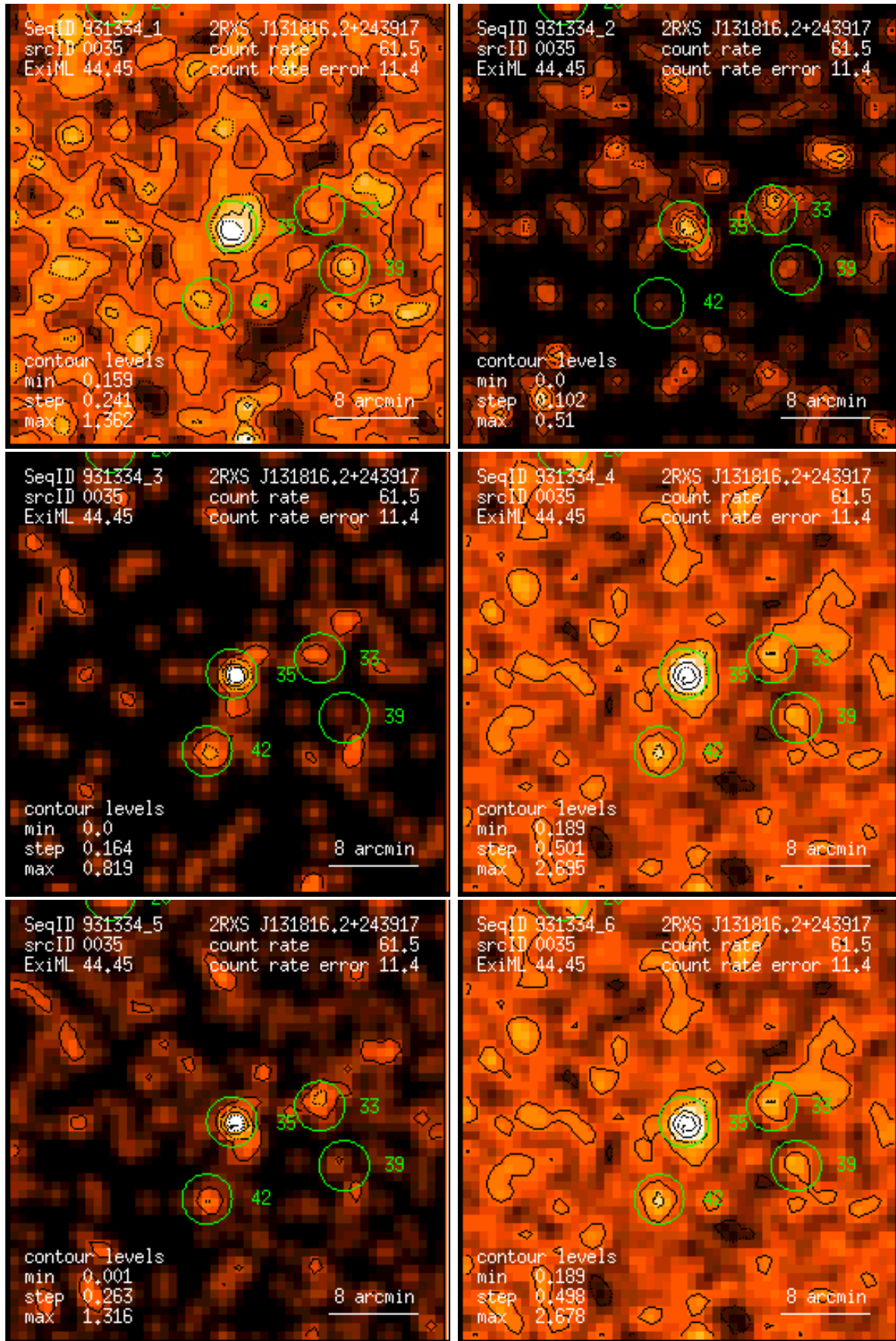
Figure 35: RASS 931334: detection 0035: band rate images, Gaussian filter: (1) PSPC channels 11 – 41, (2) 52 – 90, (3) 91 – 201, (4) 11 – 235, (5) 52 – 201, (6) 11 – 201. Broad band rates in counts/ks. Band rate contour levels in counts/ks/arcmin 2 .
