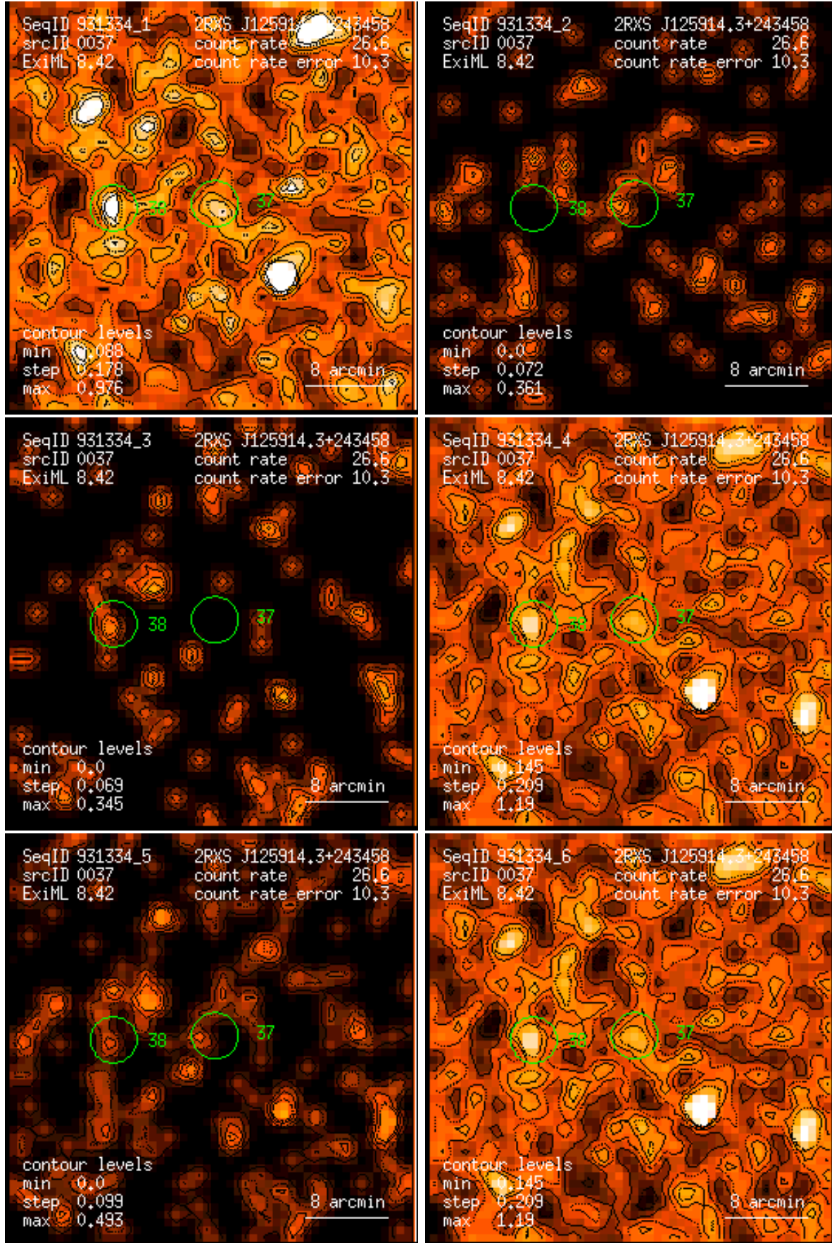
Figure 37: RASS 931334: detection 0037: band rate images, Gaussian filter: (1) PSPC channels 11 – 41, (2) 52 – 90, (3) 91 – 201, (4) 11 – 235, (5) 52 – 201, (6) 11 – 201. Broad band rates in counts/ks. Band rate contour levels in counts/ks/arcmin 2 .
