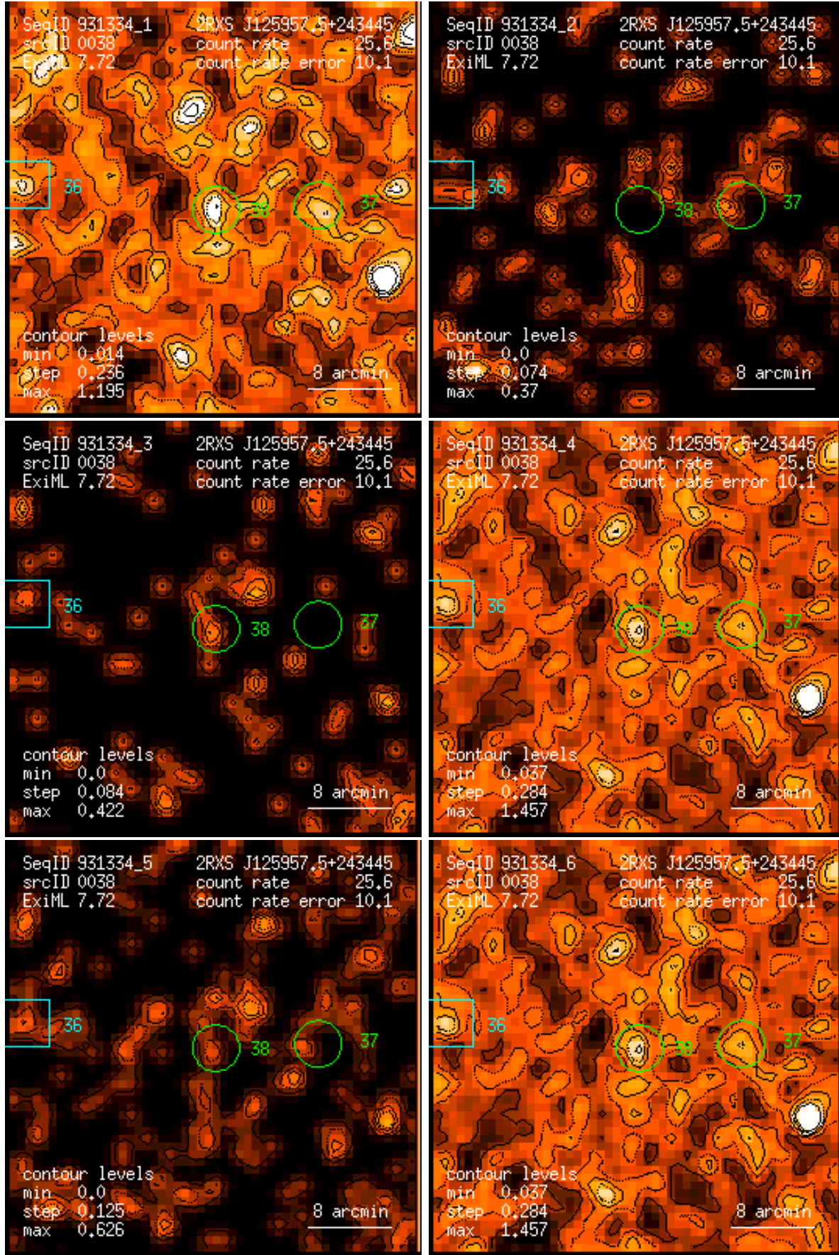
Figure 38: RASS 931334: detection 0038: band rate images, Gaussian filter: (1) PSPC channels 11 – 41, (2) 52 – 90, (3) 91 – 201, (4) 11 – 235, (5) 52 – 201, (6) 11 – 201. Broad band rates in counts/ks. Band rate contour levels in counts/ks/arcmin 2 .
