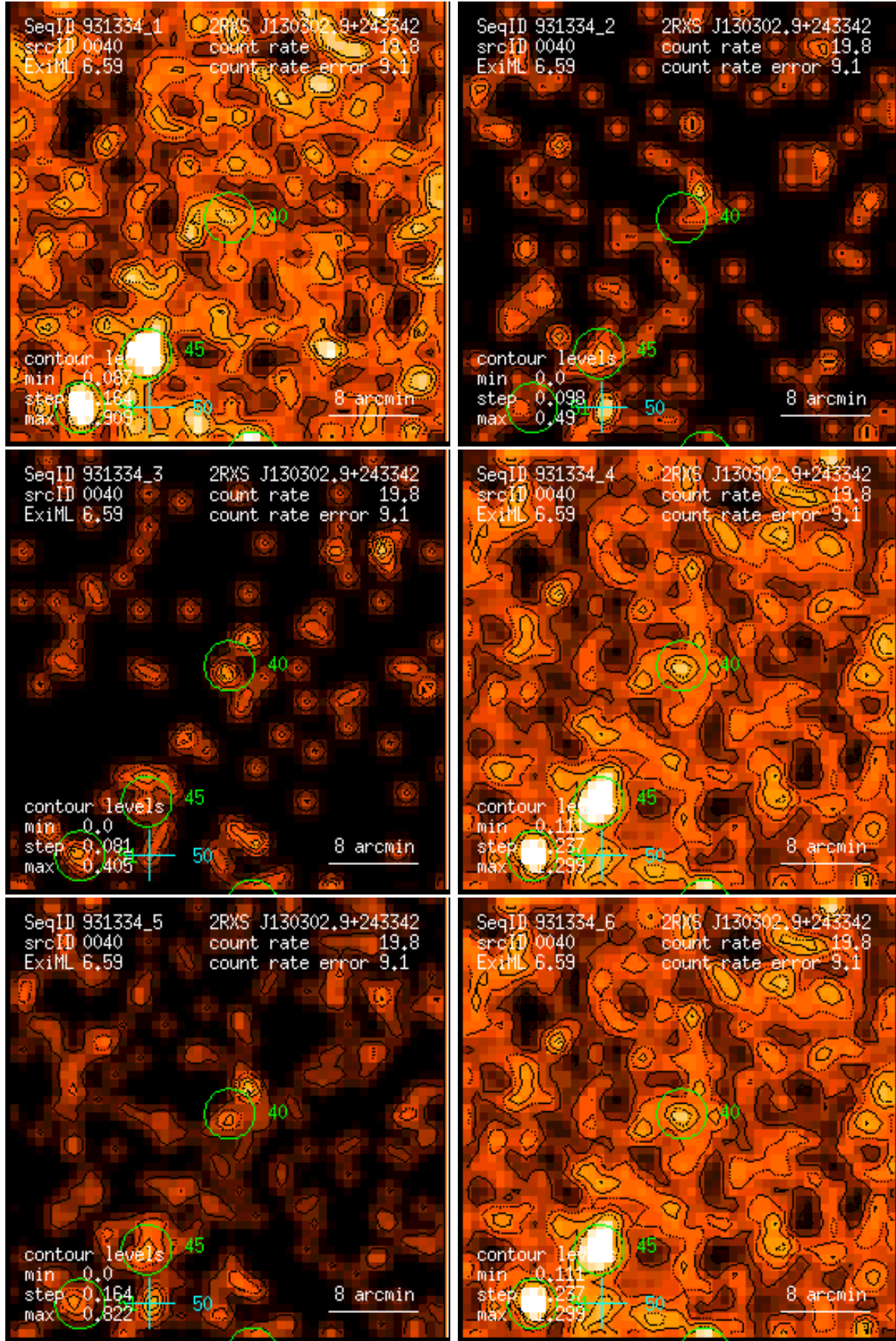
Figure 40: RASS 931334: detection 0040: band rate images, Gaussian filter: (1) PSPC channels 11 – 41, (2) 52 – 90, (3) 91 – 201, (4) 11 – 235, (5) 52 – 201, (6) 11 – 201. Broad band rates in counts/ks. Band rate contour levels in counts/ks/arcmin 2 .
