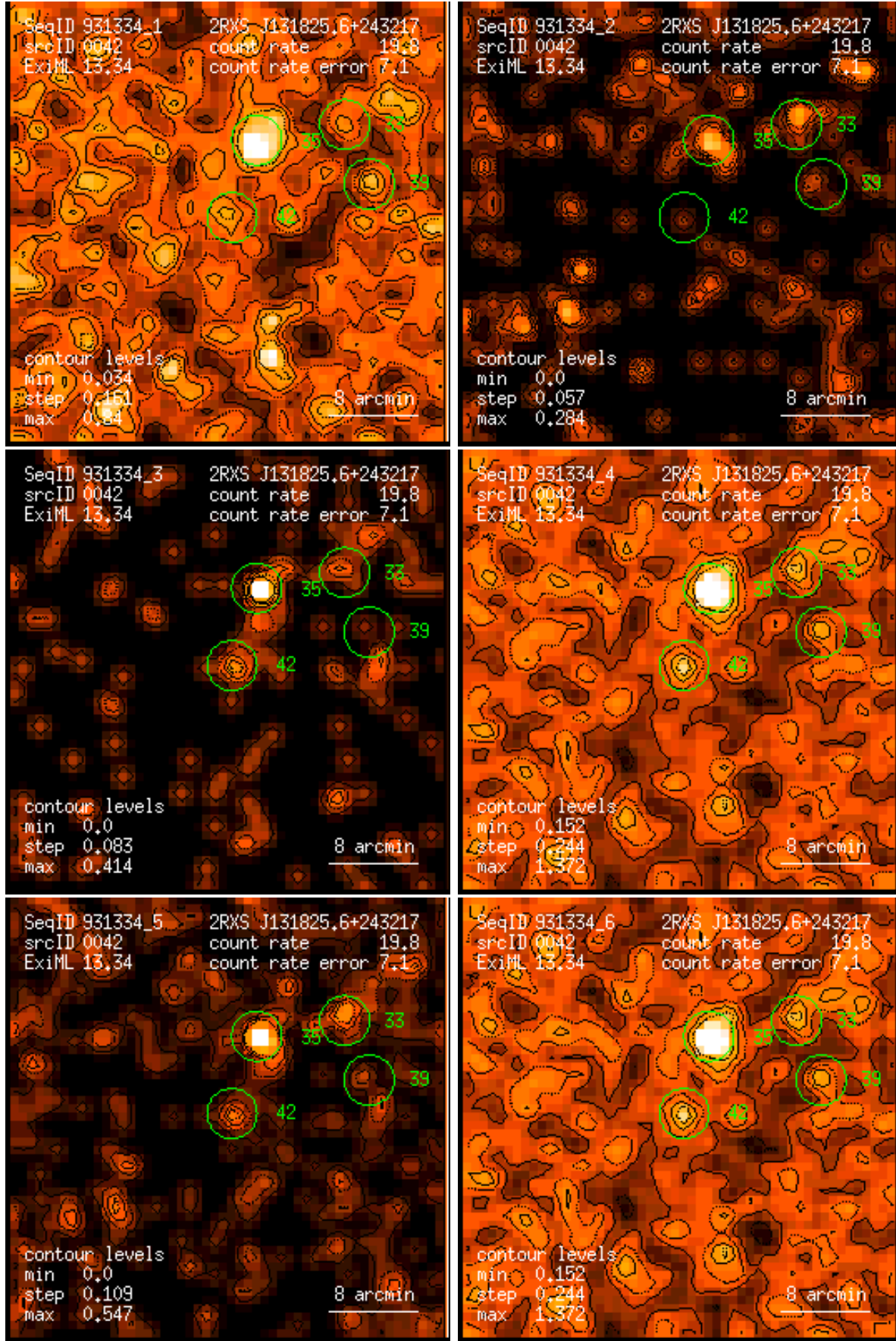
Figure 42: RASS 931334: detection 0042: band rate images, Gaussian filter: (1) PSPC channels 11 – 41, (2) 52 – 90, (3) 91 – 201, (4) 11 – 235, (5) 52 – 201, (6) 11 – 201. Broad band rates in counts/ks. Band rate contour levels in counts/ks/arcmin 2 .
