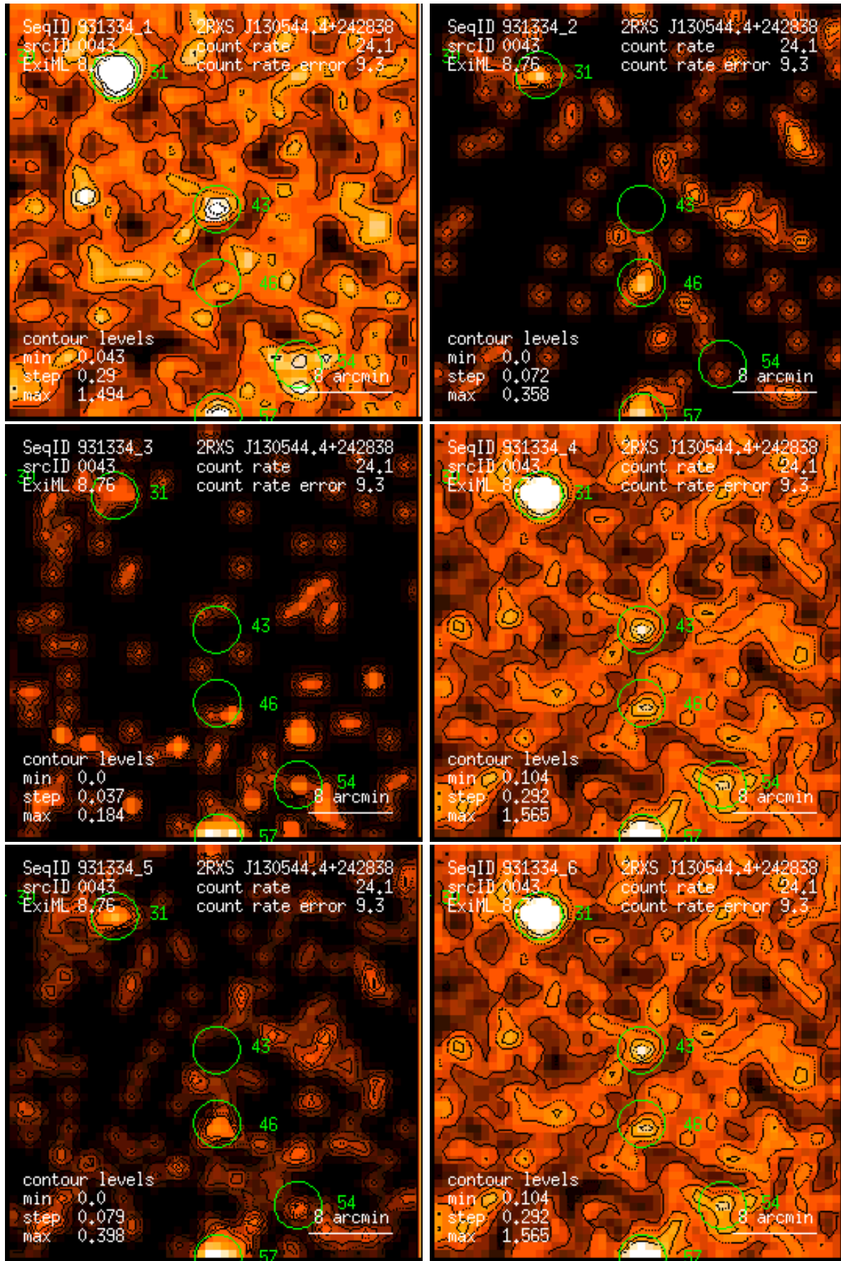
Figure 43: RASS 931334: detection 0043: band rate images, Gaussian filter: (1) PSPC channels 11 – 41, (2) 52 – 90, (3) 91 – 201, (4) 11 – 235, (5) 52 – 201, (6) 11 – 201. Broad band rates in counts/ks. Band rate contour levels in counts/ks/arcmin 2 .
