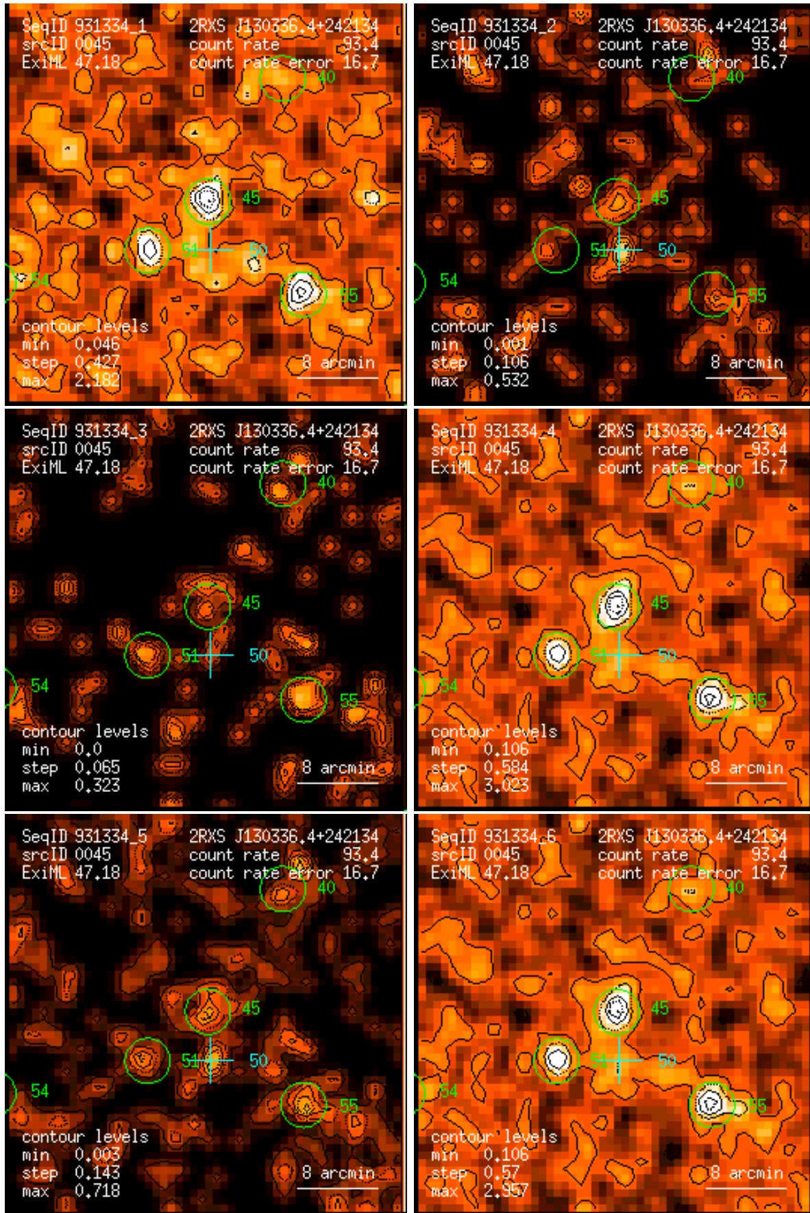
Figure 45: RASS 931334: detection 0045: band rate images, Gaussian filter: (1) PSPC channels 11 – 41, (2) 52 – 90, (3) 91 – 201, (4) 11 – 235, (5) 52 – 201, (6) 11 – 201. Broad band rates in counts/ks. Band rate contour levels in counts/ks/arcmin 2 .
