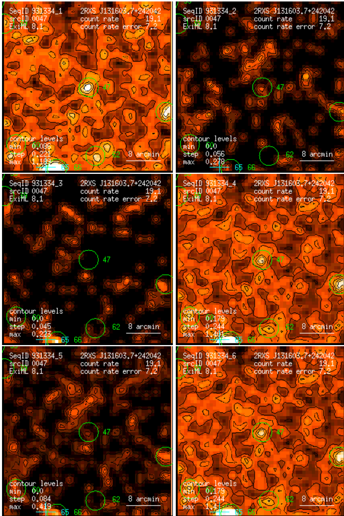
Figure 47: RASS 931334: detection 0047: band rate images, Gaussian filter: (1) PSPC channels 11 – 41, (2) 52 – 90, (3) 91 – 201, (4) 11 – 235, (5) 52 – 201, (6) 11 – 201. Broad band rates in counts/ks. Band rate contour levels in counts/ks/arcmin 2 .
