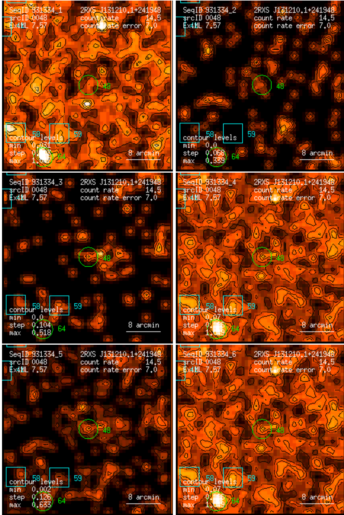
Figure 48: RASS 931334: detection 0048: band rate images, Gaussian filter: (1) PSPC channels 11 – 41, (2) 52 – 90, (3) 91 – 201, (4) 11 – 235, (5) 52 – 201, (6) 11 – 201. Broad band rates in counts/ks. Band rate contour levels in counts/ks/arcmin 2 .
