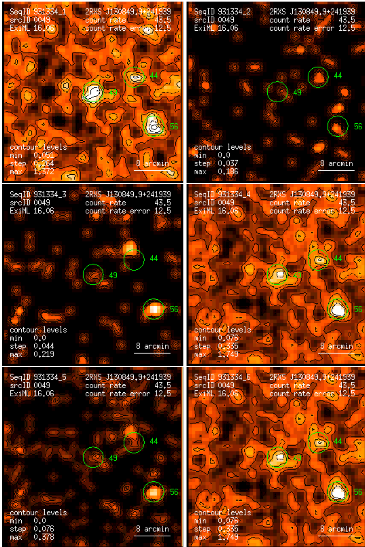
Figure 49: RASS 931334: detection 0049: band rate images, Gaussian filter: (1) PSPC channels 11 – 41, (2) 52 – 90, (3) 91 – 201, (4) 11 – 235, (5) 52 – 201, (6) 11 – 201. Broad band rates in counts/ks. Band rate contour levels in counts/ks/arcmin 2 .
