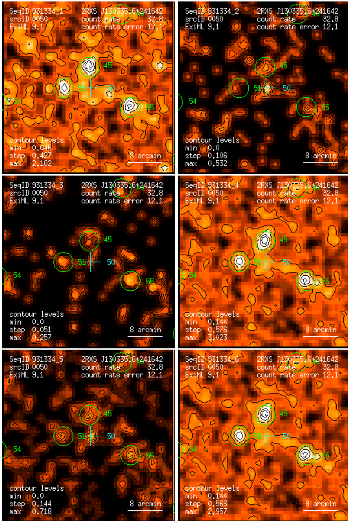
Figure 50: RASS 931334: detection 0050: band rate images, Gaussian filter: (1) PSPC channels 11 – 41, (2) 52 – 90, (3) 91 – 201, (4) 11 – 235, (5) 52 – 201, (6) 11 – 201. Broad band rates in counts/ks. Band rate contour levels in counts/ks/arcmin 2 .
