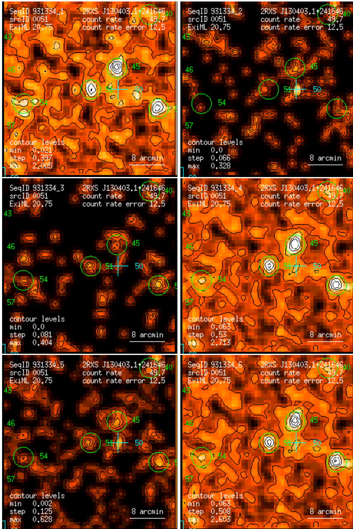
Figure 51: RASS 931334: detection 0051: band rate images, Gaussian filter: (1) PSPC channels 11 – 41, (2) 52 – 90, (3) 91 – 201, (4) 11 – 235, (5) 52 – 201, (6) 11 – 201. Broad band rates in counts/ks. Band rate contour levels in counts/ks/arcmin 2 .
