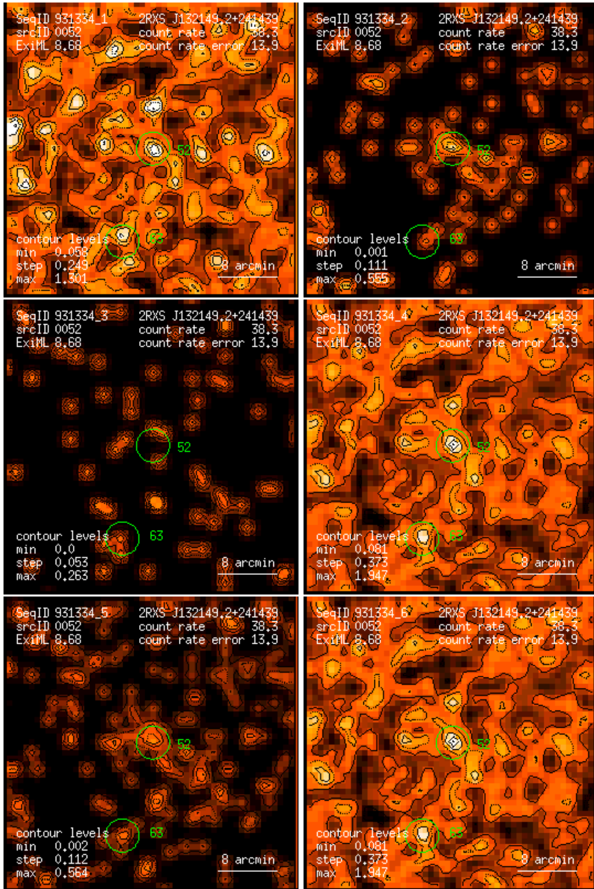
Figure 52: RASS 931334: detection 0052: band rate images, Gaussian filter: (1) PSPC channels 11 – 41, (2) 52 – 90, (3) 91 – 201, (4) 11 – 235, (5) 52 – 201, (6) 11 – 201. Broad band rates in counts/ks. Band rate contour levels in counts/ks/arcmin 2 .
