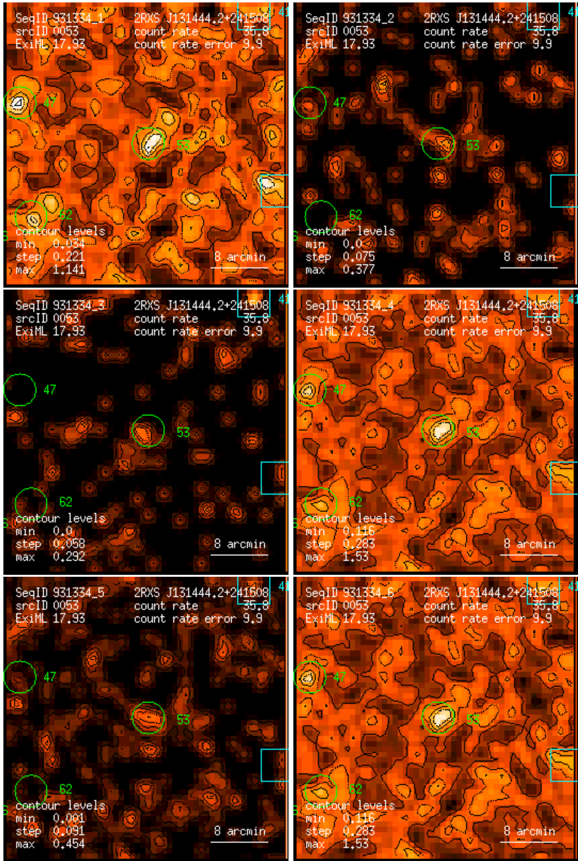
Figure 53: RASS 931334: detection 0053: band rate images, Gaussian filter: (1) PSPC channels 11 – 41, (2) 52 – 90, (3) 91 – 201, (4) 11 – 235, (5) 52 – 201, (6) 11 – 201. Broad band rates in counts/ks. Band rate contour levels in counts/ks/arcmin 2 .
