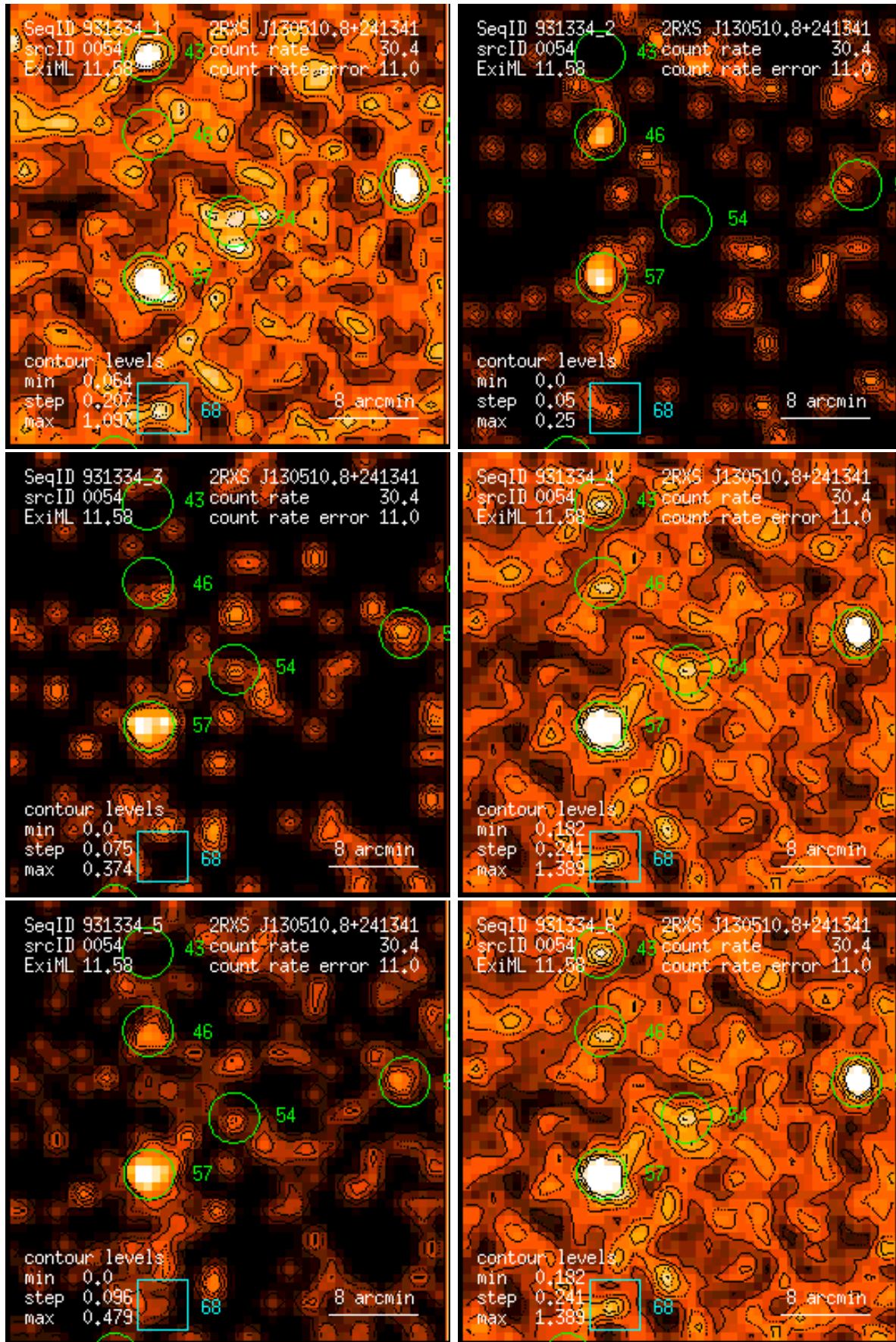
Figure 54: RASS 931334: detection 0054: band rate images, Gaussian filter: (1) PSPC channels 11 – 41, (2) 52 – 90, (3) 91 – 201, (4) 11 – 235, (5) 52 – 201, (6) 11 – 201. Broad band rates in counts/ks. Band rate contour levels in counts/ks/arcmin 2 .
