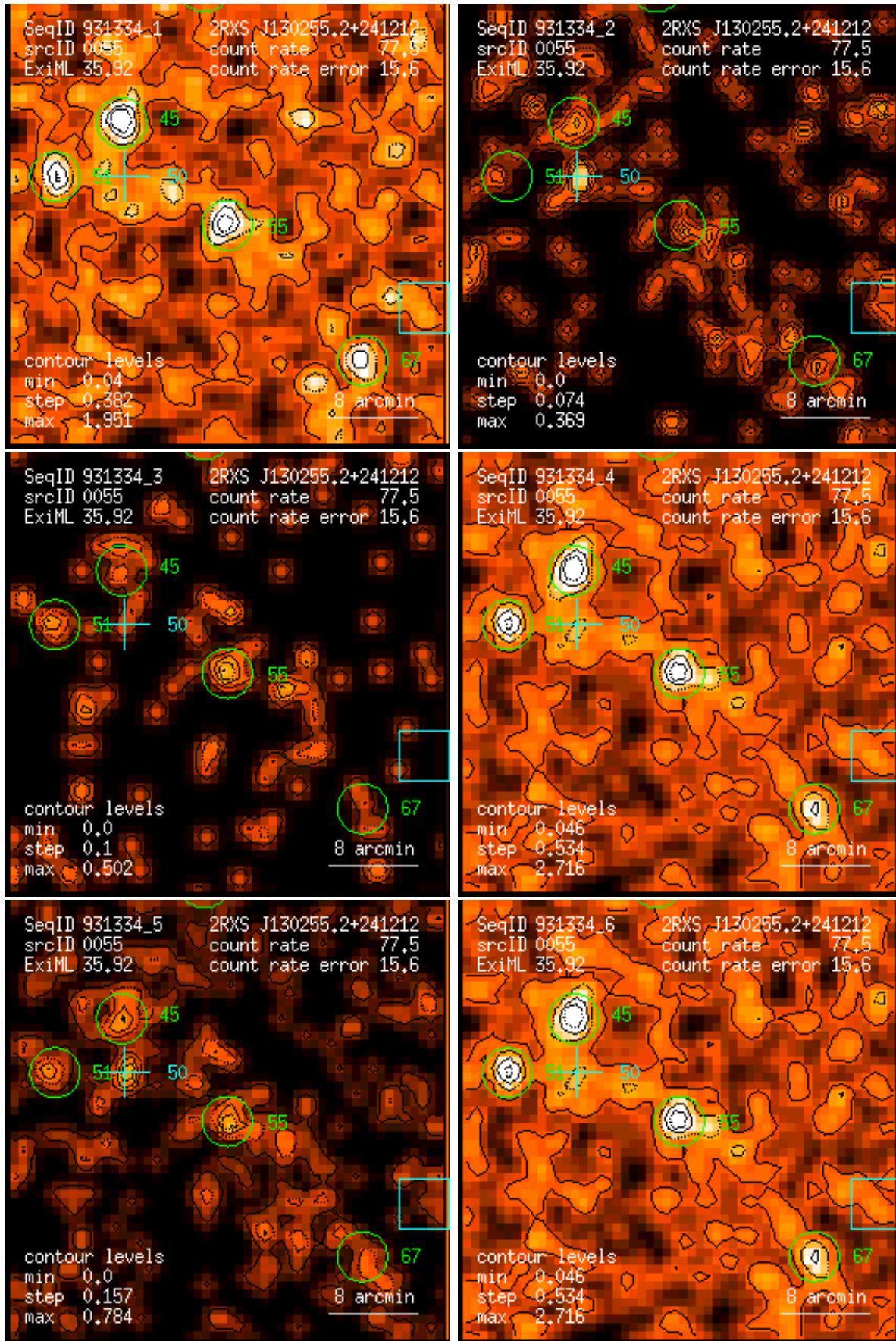
Figure 55: RASS 931334: detection 0055: band rate images, Gaussian filter: (1) PSPC channels 11 – 41, (2) 52 – 90, (3) 91 – 201, (4) 11 – 235, (5) 52 – 201, (6) 11 – 201. Broad band rates in counts/ks. Band rate contour levels in counts/ks/arcmin 2 .
