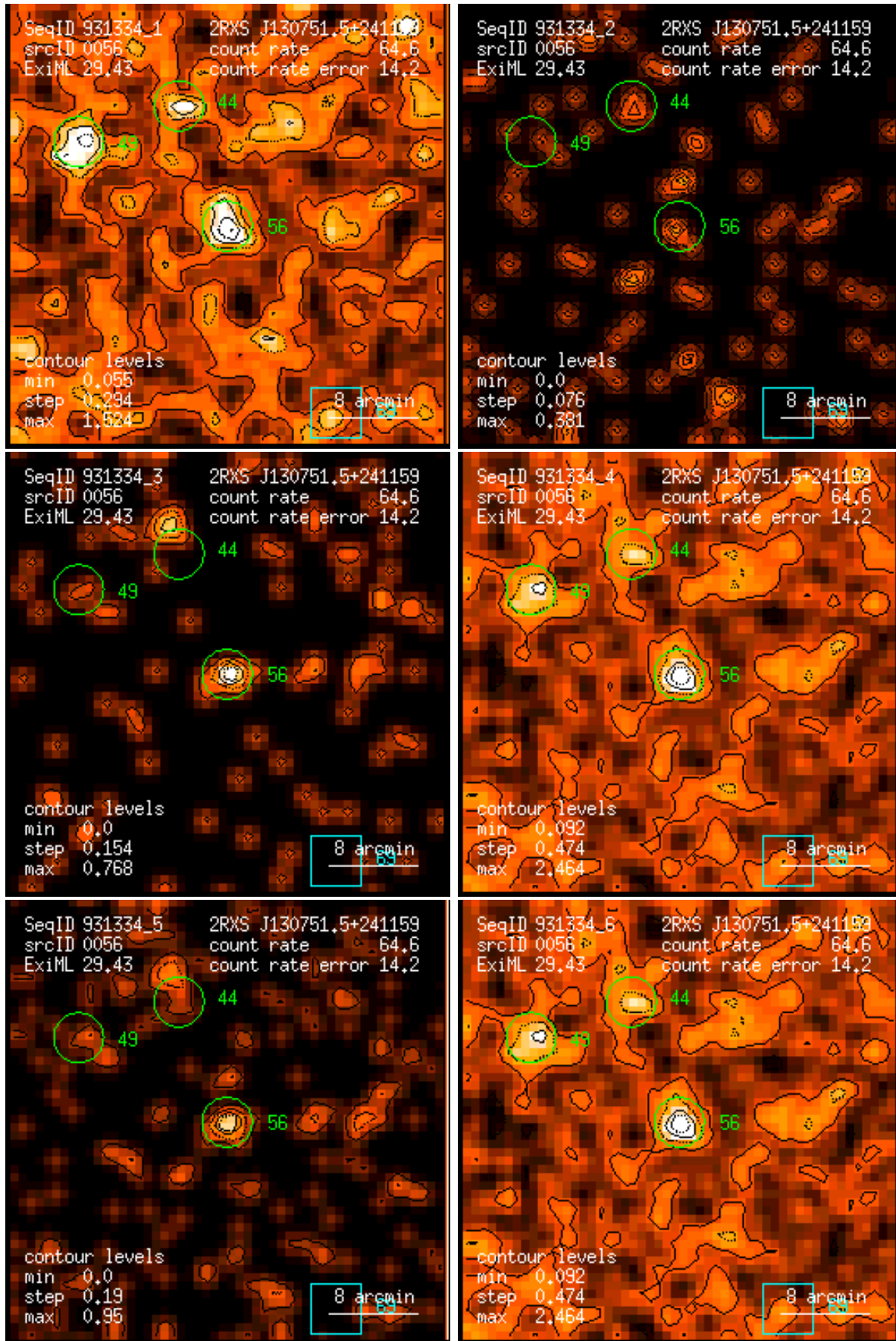
Figure 56: RASS 931334: detection 0056: band rate images, Gaussian filter: (1) PSPC channels 11 – 41, (2) 52 – 90, (3) 91 – 201, (4) 11 – 235, (5) 52 – 201, (6) 11 – 201. Broad band rates in counts/ks. Band rate contour levels in counts/ks/arcmin 2 .
