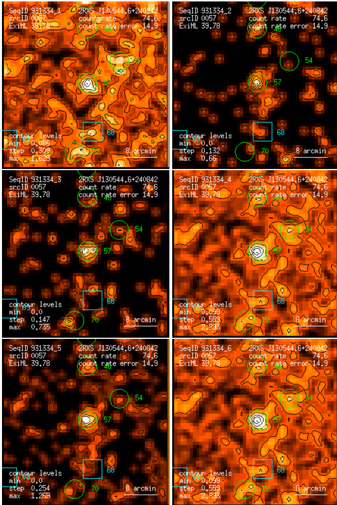
Figure 57: RASS 931334: detection 0057: band rate images, Gaussian filter: (1) PSPC channels 11 – 41, (2) 52 – 90, (3) 91 – 201, (4) 11 – 235, (5) 52 – 201, (6) 11 – 201. Broad band rates in counts/ks. Band rate contour levels in counts/ks/arcmin 2 .
