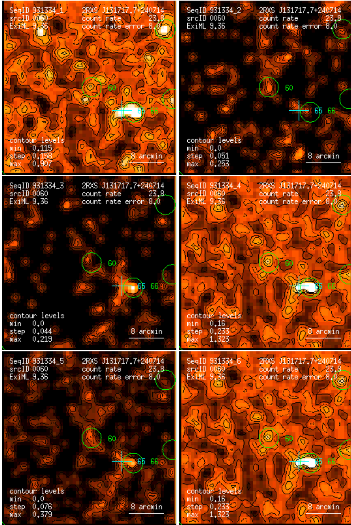
Figure 60: RASS 931334: detection 0060: band rate images, Gaussian filter: (1) PSPC channels 11 – 41, (2) 52 – 90, (3) 91 – 201, (4) 11 – 235, (5) 52 – 201, (6) 11 – 201. Broad band rates in counts/ks. Band rate contour levels in counts/ks/arcmin 2 .
