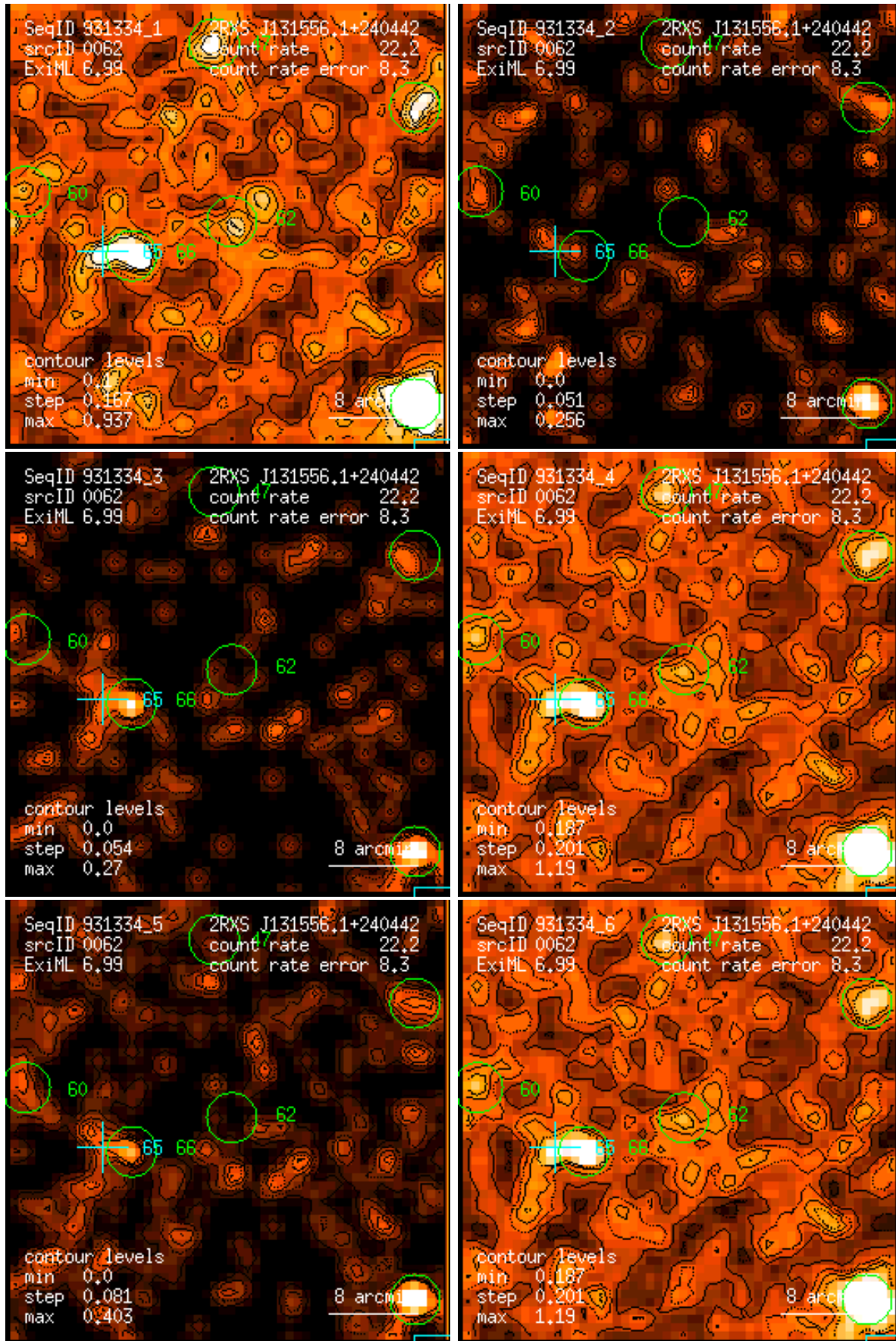
Figure 62: RASS 931334: detection 0062: band rate images, Gaussian filter: (1) PSPC channels 11 – 41, (2) 52 – 90, (3) 91 – 201, (4) 11 – 235, (5) 52 – 201, (6) 11 – 201. Broad band rates in counts/ks. Band rate contour levels in counts/ks/arcmin 2 .
