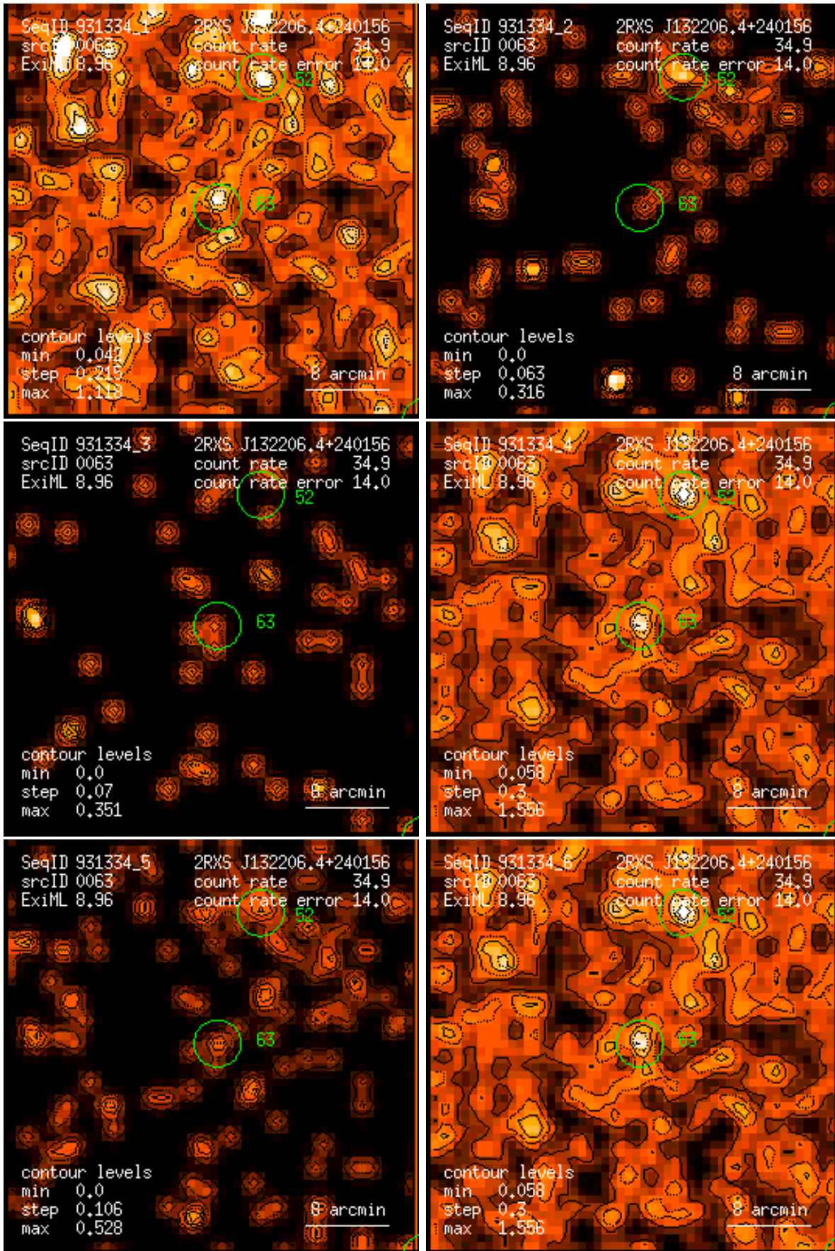
Figure 63: RASS 931334: detection 0063: band rate images, Gaussian filter: (1) PSPC channels 11 – 41, (2) 52 – 90, (3) 91 – 201, (4) 11 – 235, (5) 52 – 201, (6) 11 – 201. Broad band rates in counts/ks. Band rate contour levels in counts/ks/arcmin 2 .
