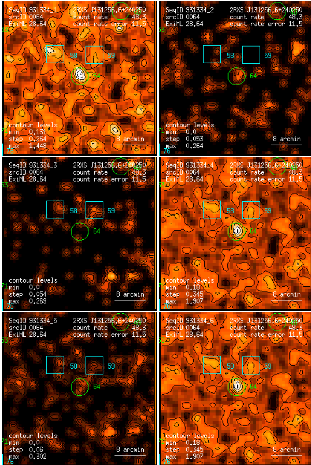
Figure 64: RASS 931334: detection 0064: band rate images, Gaussian filter: (1) PSPC channels 11 – 41, (2) 52 – 90, (3) 91 – 201, (4) 11 – 235, (5) 52 – 201, (6) 11 – 201. Broad band rates in counts/ks. Band rate contour levels in counts/ks/arcmin 2 .
