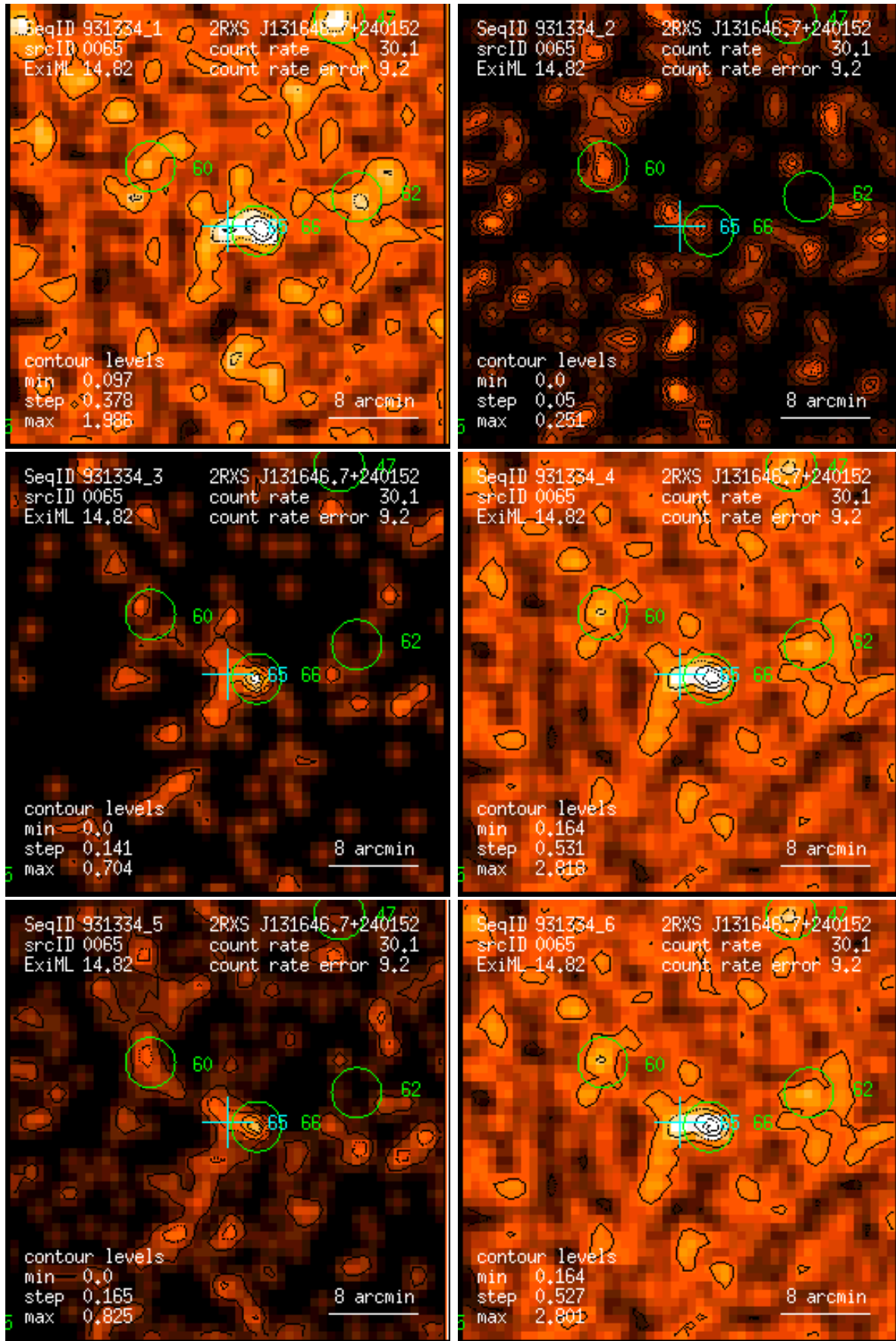
Figure 65: RASS 931334: detection 0065: band rate images, Gaussian filter: (1) PSPC channels 11 – 41, (2) 52 – 90, (3) 91 – 201, (4) 11 – 235, (5) 52 – 201, (6) 11 – 201. Broad band rates in counts/ks. Band rate contour levels in counts/ks/arcmin 2 .
