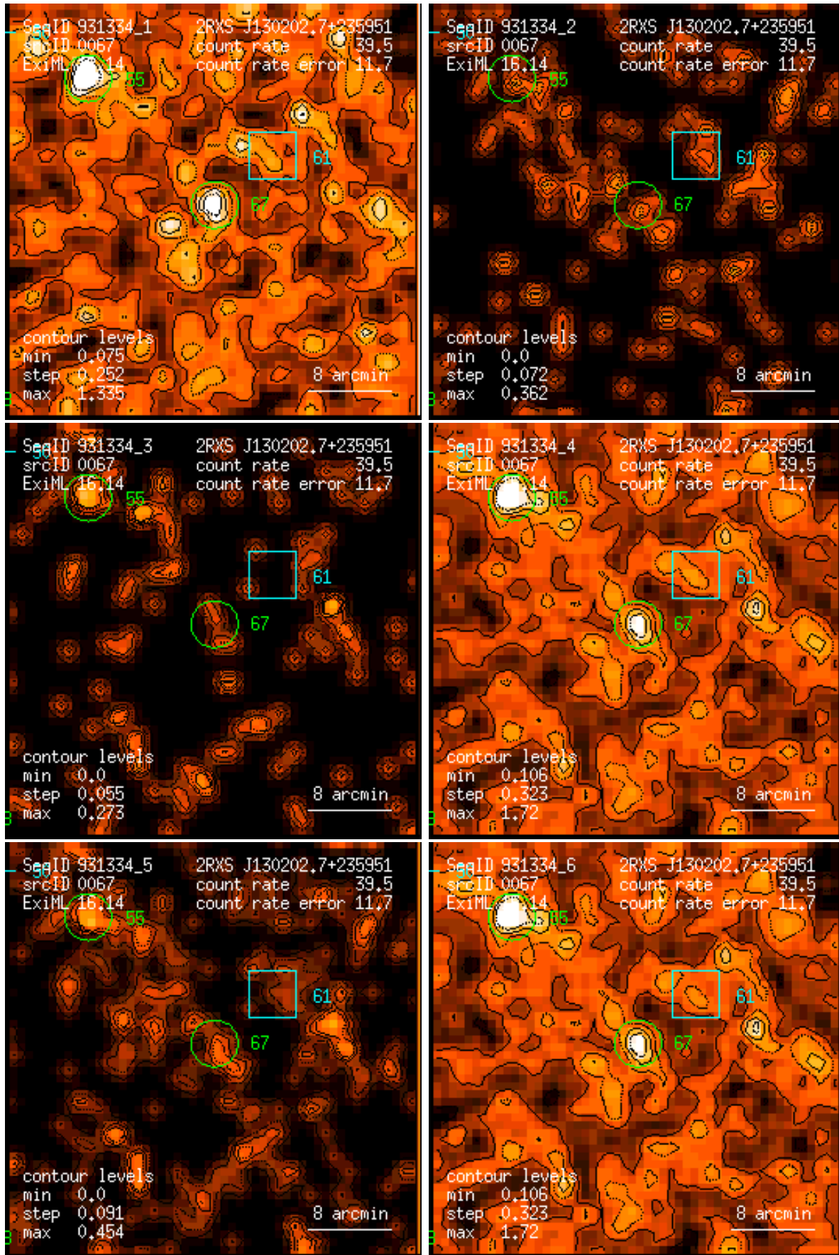
Figure 67: RASS 931334: detection 0067: band rate images, Gaussian filter: (1) PSPC channels 11 – 41, (2) 52 – 90, (3) 91 – 201, (4) 11 – 235, (5) 52 – 201, (6) 11 – 201. Broad band rates in counts/ks. Band rate contour levels in counts/ks/arcmin 2 .
