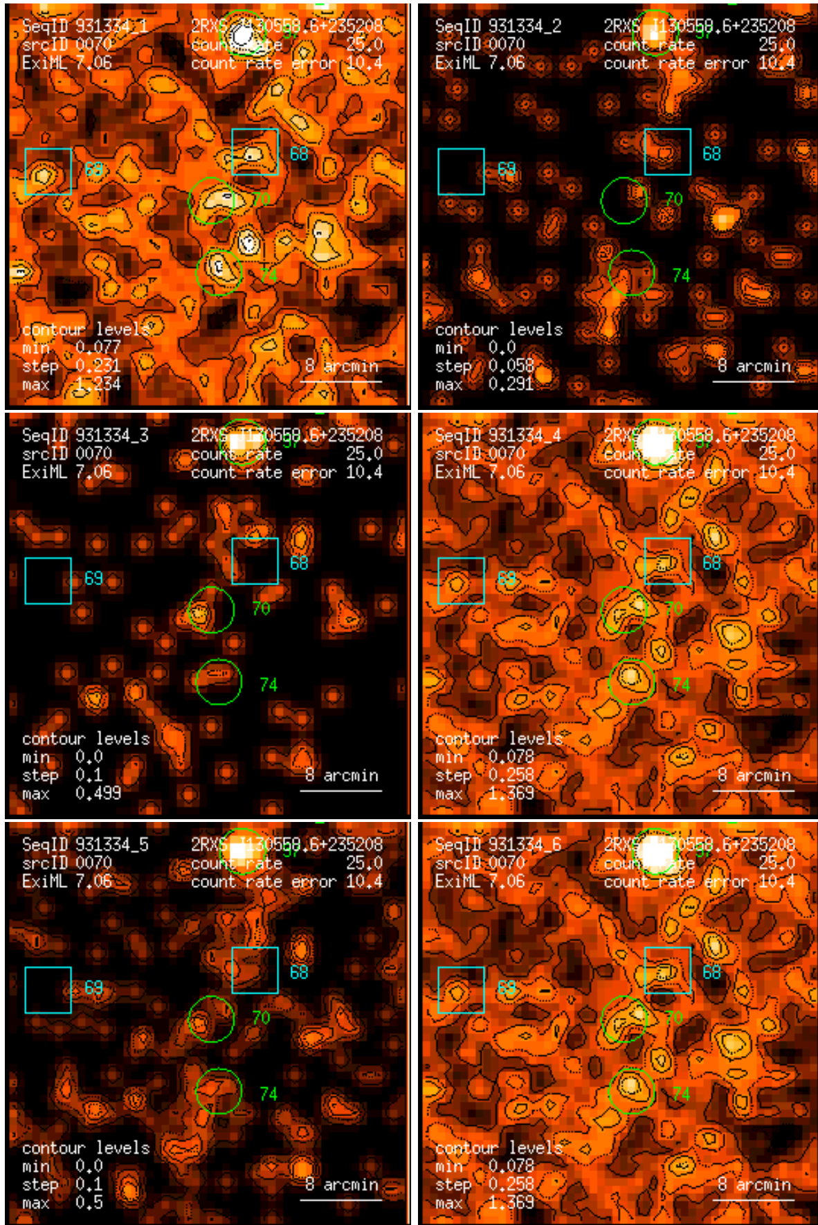
Figure 70: RASS 931334: detection 0070: band rate images, Gaussian filter: (1) PSPC channels 11 – 41, (2) 52 – 90, (3) 91 – 201, (4) 11 – 235, (5) 52 – 201, (6) 11 – 201. Broad band rates in counts/ks. Band rate contour levels in counts/ks/arcmin 2 .
