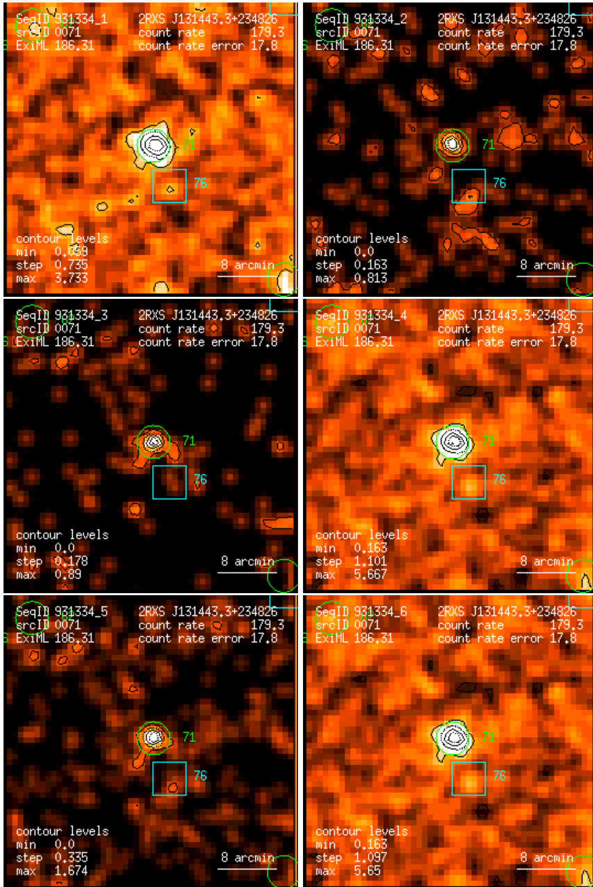
Figure 71: RASS 931334: detection 0071: band rate images, Gaussian filter: (1) PSPC channels 11 – 41, (2) 52 – 90, (3) 91 – 201, (4) 11 – 235, (5) 52 – 201, (6) 11 – 201. Broad band rates in counts/ks. Band rate contour levels in counts/ks/arcmin 2 .
