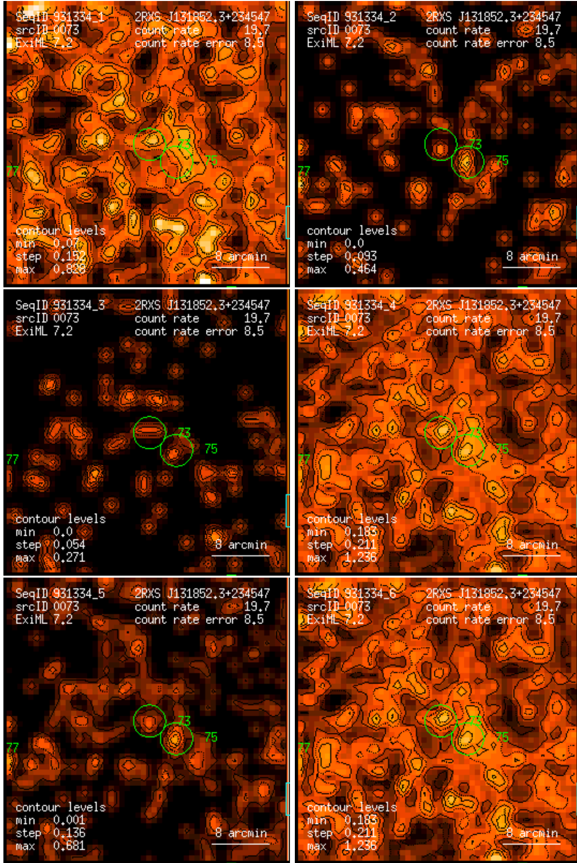
Figure 73: RASS 931334: detection 0073: band rate images, Gaussian filter: (1) PSPC channels 11 – 41, (2) 52 – 90, (3) 91 – 201, (4) 11 – 235, (5) 52 – 201, (6) 11 – 201. Broad band rates in counts/ks. Band rate contour levels in counts/ks/arcmin 2 .
