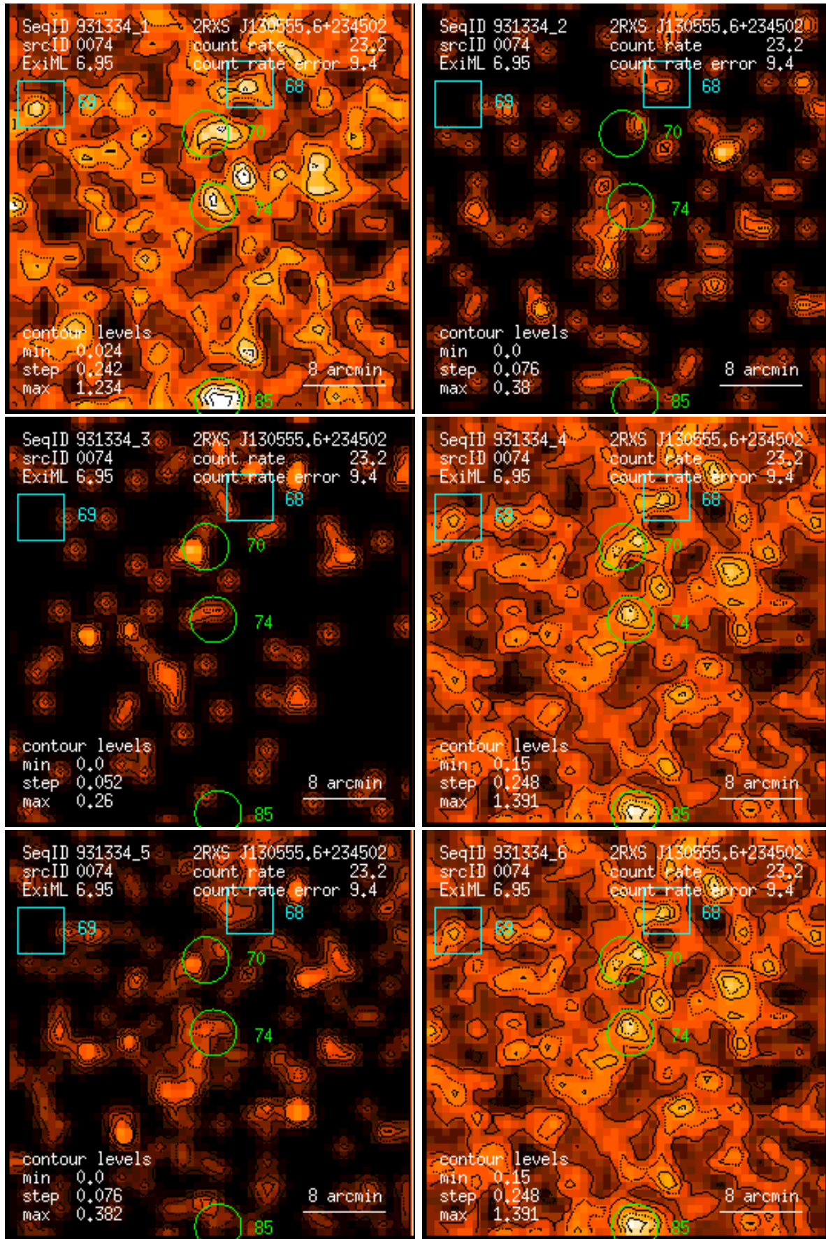
Figure 74: RASS 931334: detection 0074: band rate images, Gaussian filter: (1) PSPC channels 11 – 41, (2) 52 – 90, (3) 91 – 201, (4) 11 – 235, (5) 52 – 201, (6) 11 – 201. Broad band rates in counts/ks. Band rate contour levels in counts/ks/arcmin 2 .
