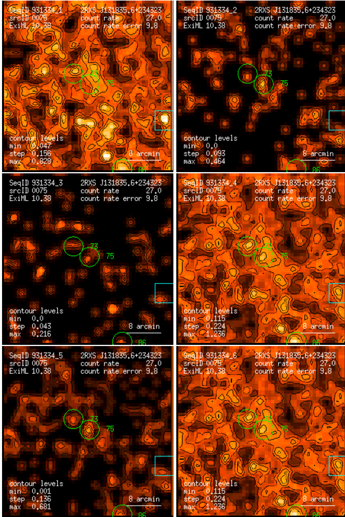
Figure 75: RASS 931334: detection 0075: band rate images, Gaussian filter: (1) PSPC channels 11 – 41, (2) 52 – 90, (3) 91 – 201, (4) 11 – 235, (5) 52 – 201, (6) 11 – 201. Broad band rates in counts/ks. Band rate contour levels in counts/ks/arcmin 2 .
