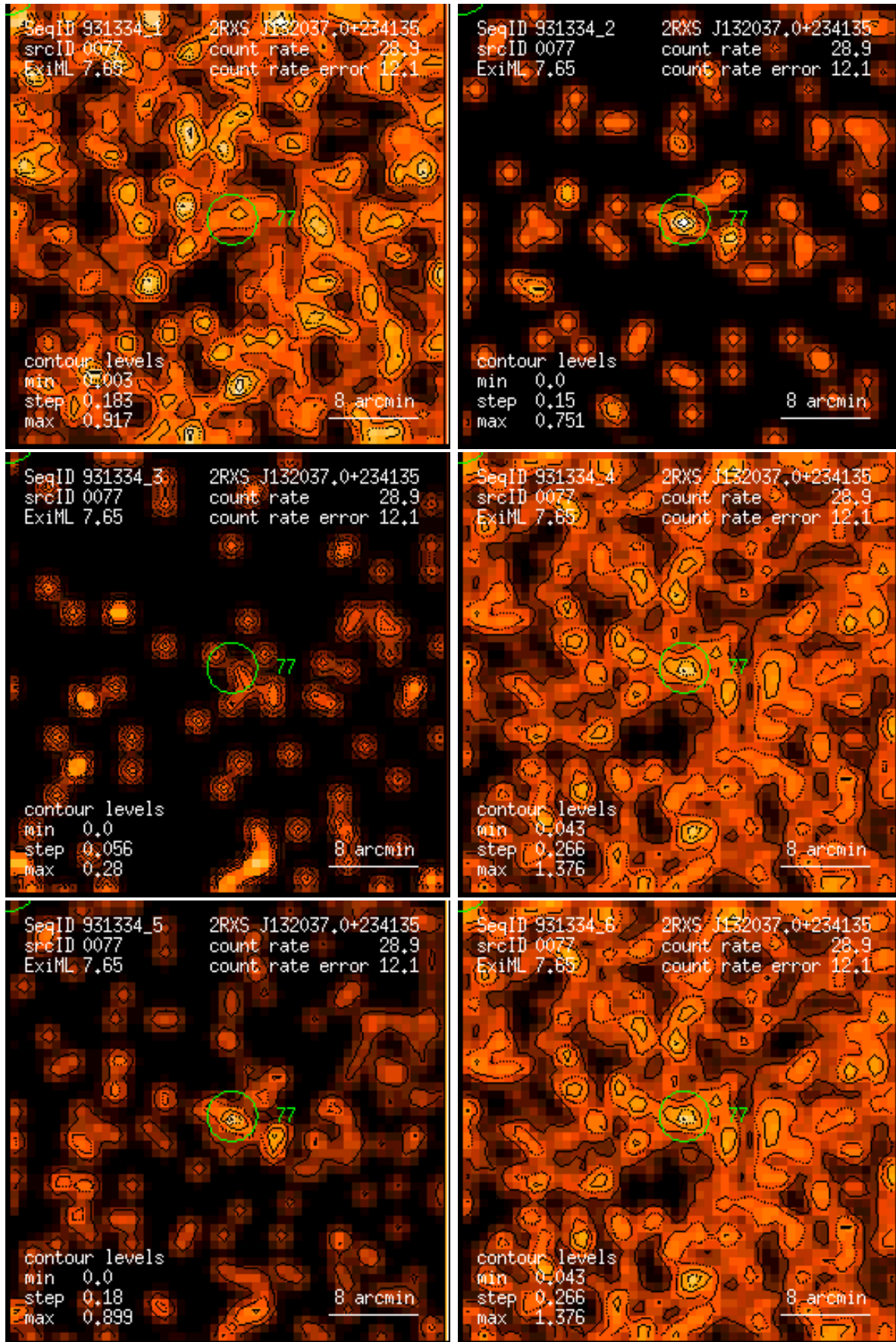
Figure 77: RASS 931334: detection 0077: band rate images, Gaussian filter: (1) PSPC channels 11 – 41, (2) 52 – 90, (3) 91 – 201, (4) 11 – 235, (5) 52 – 201, (6) 11 – 201. Broad band rates in counts/ks. Band rate contour levels in counts/ks/arcmin 2 .
