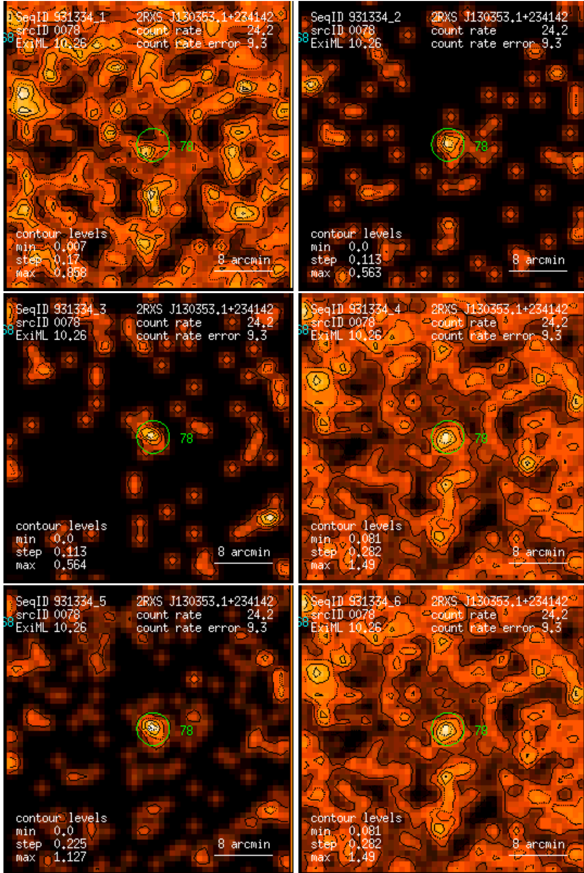
Figure 78: RASS 931334: detection 0078: band rate images, Gaussian filter: (1) PSPC channels 11 – 41, (2) 52 – 90, (3) 91 – 201, (4) 11 – 235, (5) 52 – 201, (6) 11 – 201. Broad band rates in counts/ks. Band rate contour levels in counts/ks/arcmin 2 .
