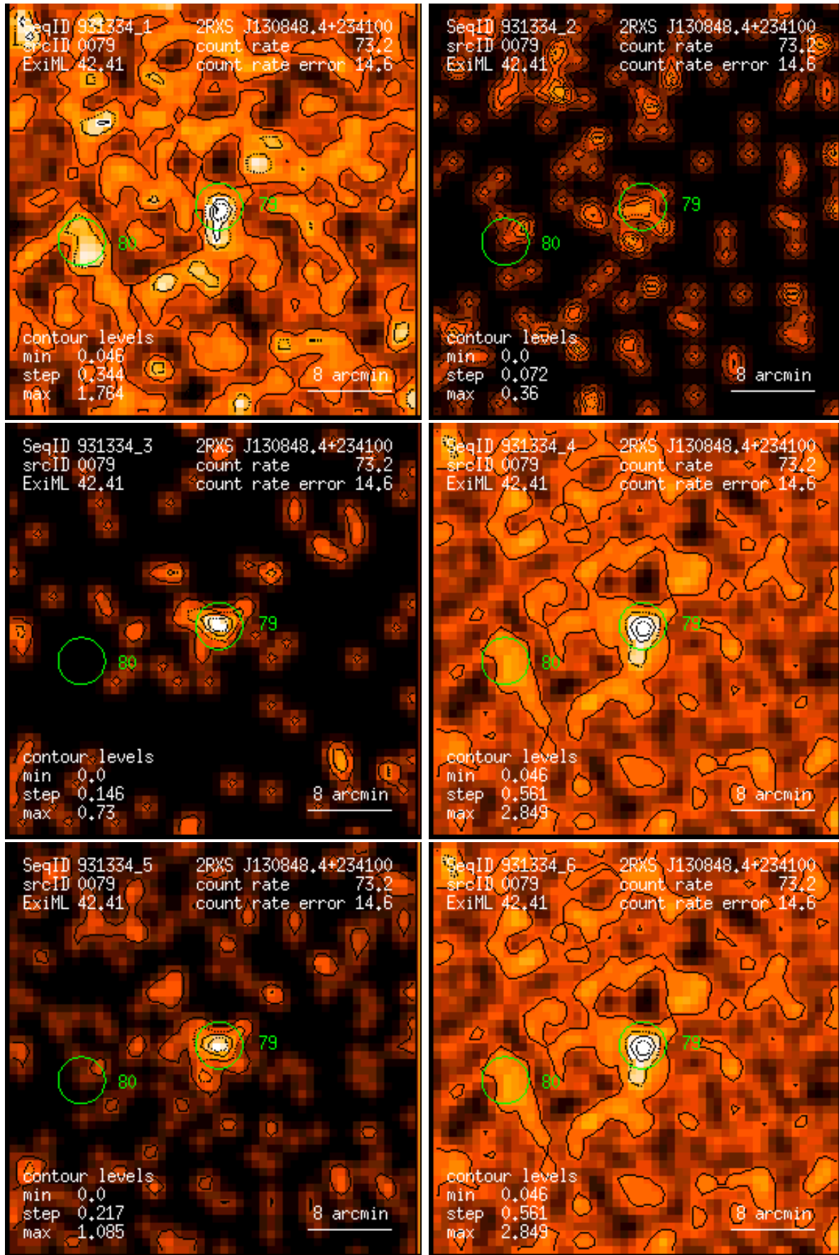
Figure 79: RASS 931334: detection 0079: band rate images, Gaussian filter: (1) PSPC channels 11 – 41, (2) 52 – 90, (3) 91 – 201, (4) 11 – 235, (5) 52 – 201, (6) 11 – 201. Broad band rates in counts/ks. Band rate contour levels in counts/ks/arcmin 2 .
