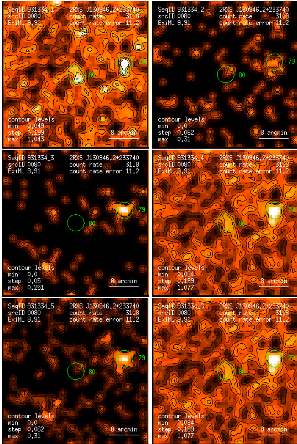
Figure 80: RASS 931334: detection 0080: band rate images, Gaussian filter: (1) PSPC channels 11 – 41, (2) 52 – 90, (3) 91 – 201, (4) 11 – 235, (5) 52 – 201, (6) 11 – 201. Broad band rates in counts/ks. Band rate contour levels in counts/ks/arcmin 2 .
