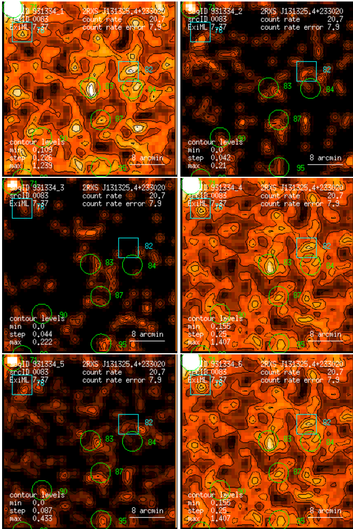
Figure 83: RASS 931334: detection 0083: band rate images, Gaussian filter: (1) PSPC channels 11 – 41, (2) 52 – 90, (3) 91 – 201, (4) 11 – 235, (5) 52 – 201, (6) 11 – 201. Broad band rates in counts/ks. Band rate contour levels in counts/ks/arcmin 2 .
