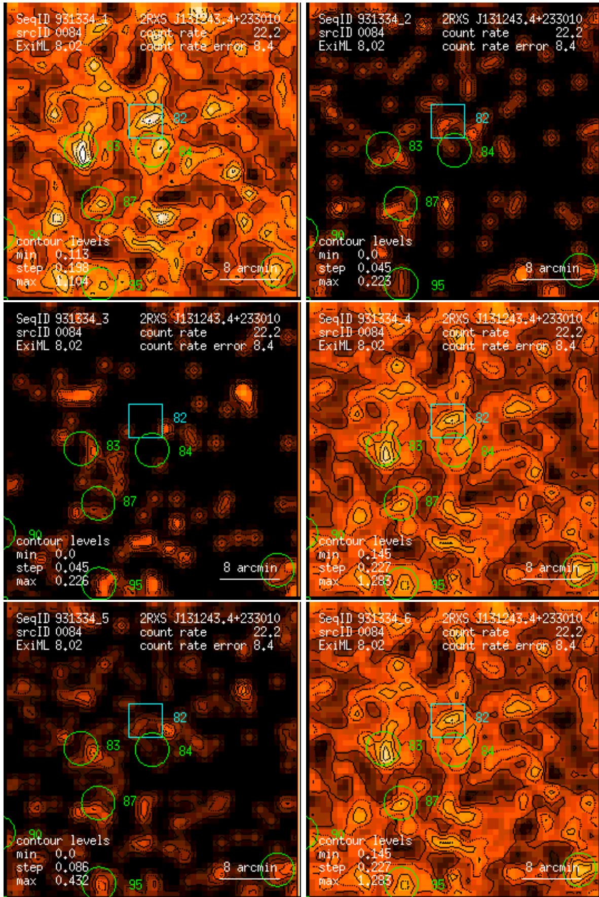
Figure 84: RASS 931334: detection 0084: band rate images, Gaussian filter: (1) PSPC channels 11 – 41, (2) 52 – 90, (3) 91 – 201, (4) 11 – 235, (5) 52 – 201, (6) 11 – 201. Broad band rates in counts/ks. Band rate contour levels in counts/ks/arcmin 2 .
