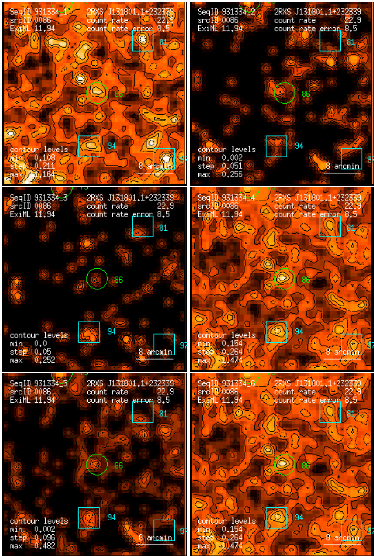
Figure 86: RASS 931334: detection 0086: band rate images, Gaussian filter: (1) PSPC channels 11 – 41, (2) 52 – 90, (3) 91 – 201, (4) 11 – 235, (5) 52 – 201, (6) 11 – 201. Broad band rates in counts/ks. Band rate contour levels in counts/ks/arcmin 2 .
