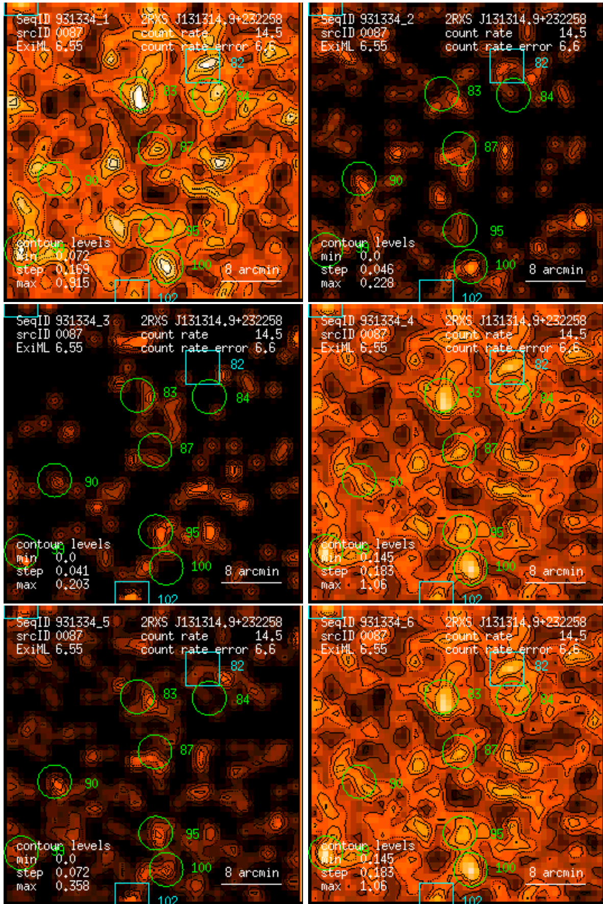
Figure 87: RASS 931334: detection 0087: band rate images, Gaussian filter: (1) PSPC channels 11 – 41, (2) 52 – 90, (3) 91 – 201, (4) 11 – 235, (5) 52 – 201, (6) 11 – 201. Broad band rates in counts/ks. Band rate contour levels in counts/ks/arcmin 2 .
