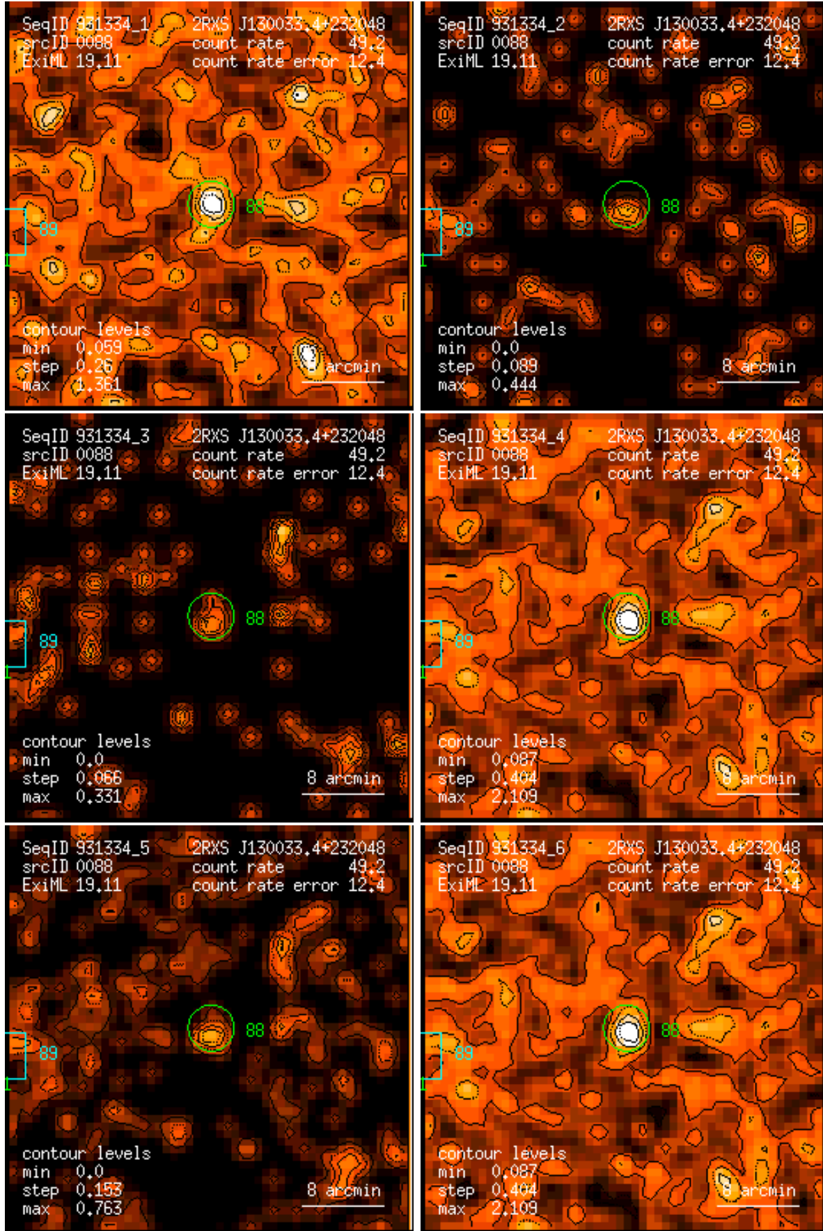
Figure 88: RASS 931334: detection 0088: band rate images, Gaussian filter: (1) PSPC channels 11 – 41, (2) 52 – 90, (3) 91 – 201, (4) 11 – 235, (5) 52 – 201, (6) 11 – 201. Broad band rates in counts/ks. Band rate contour levels in counts/ks/arcmin 2 .
