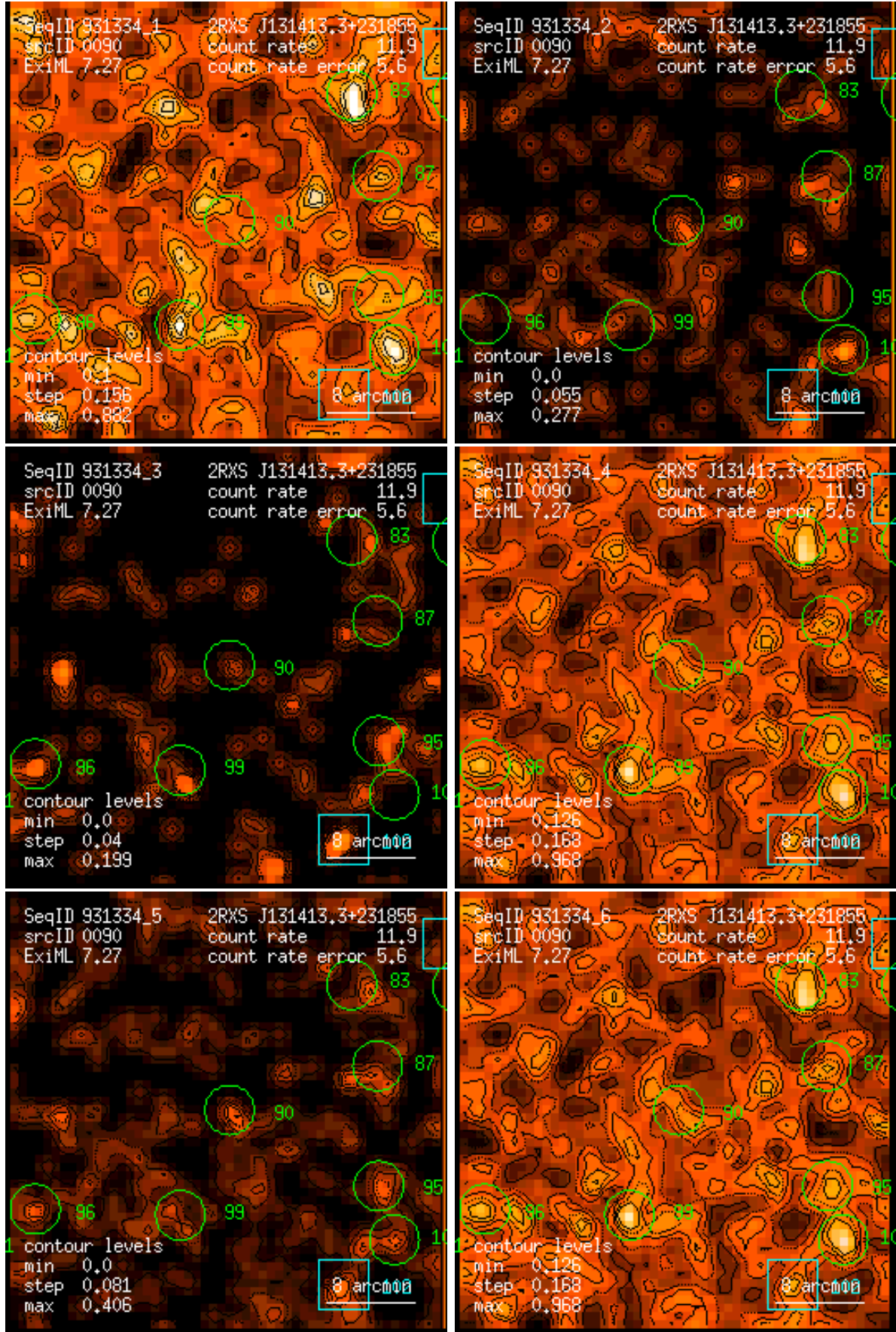
Figure 90: RASS 931334: detection 0090: band rate images, Gaussian filter: (1) PSPC channels 11 – 41, (2) 52 – 90, (3) 91 – 201, (4) 11 – 235, (5) 52 – 201, (6) 11 – 201. Broad band rates in counts/ks. Band rate contour levels in counts/ks/arcmin 2 .
